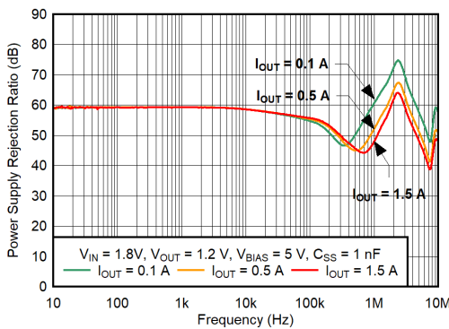
New chip
