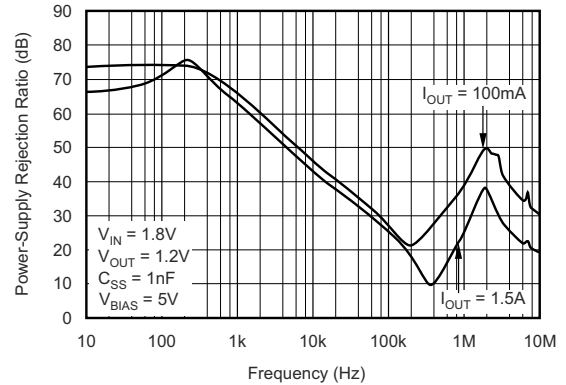
Legacy chip
