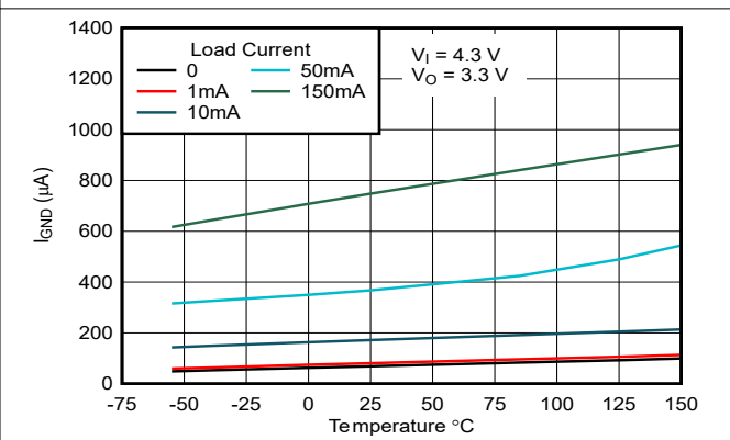
Figure 5-18. Ground-Pin Current vs Temperature (new chip)
