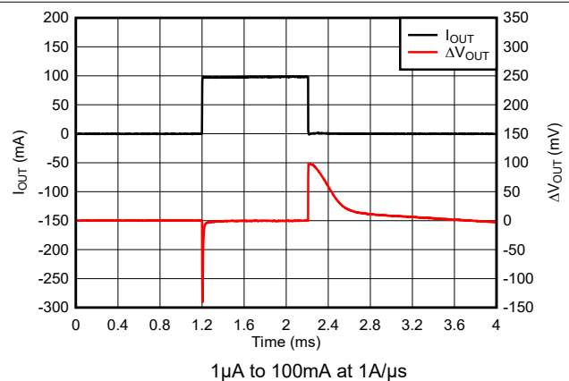
Figure 7-15. TPS76933 Load Transient Response (New Chip)
