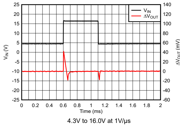
Figure 7-12. TPS76933 Line Transient Response (New Chip)
