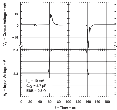
Figure 7-10. TPS76933 Line Transient Response (Legacy Chip)
