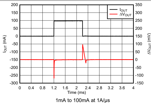
Figure 7-14. TPS76933 Load Transient Response (New Chip)
