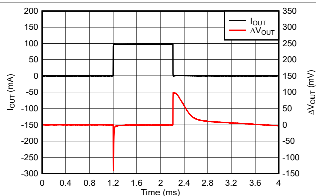
Figure 5-44. TPS76933 Load Transient Response (New Chip)
