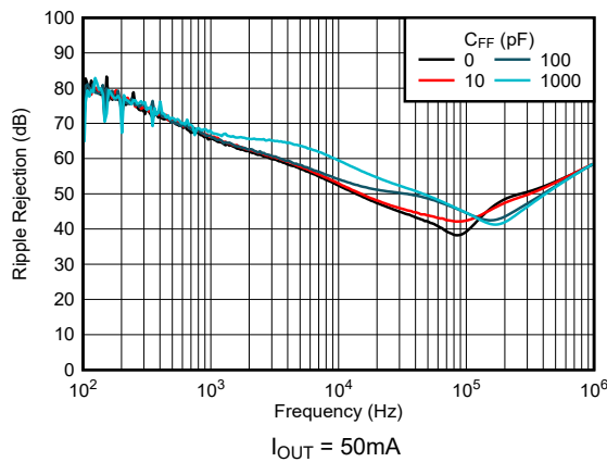
Figure 5-33. TPS76901-Q1 Ripple Rejection vs Feed-Forward Capacitor (New Chip)
