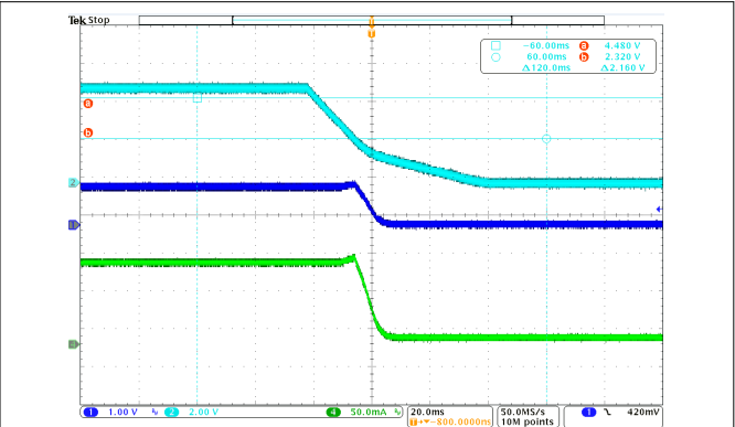
Channel 1 = V_{OUT} , channel 2 = V_{IN} , channel 4 = I_{OUT}
