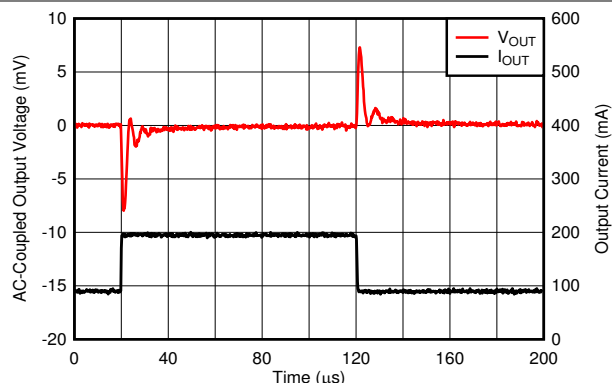
Figure 6-51. Load Transient
