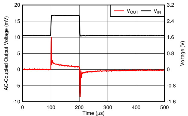
V_{\text{OUT}} = 1.2\text{ V} , I_{\text{OUT}} = 300\text{ mA} , slew rate = 1\text{ V}/\mu\text{s} , T_J = 150^\circ\text{C}
