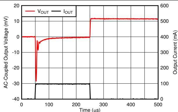
Figure 6-49. Load Transient
