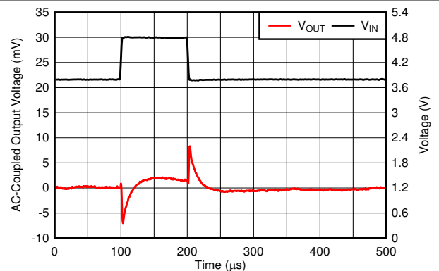
V_{\text{OUT}} = 3.3\text{ V} , I_{\text{OUT}} = 50\text{ mA} , slew rate = 1\text{ V}/\mu\text{s} , T_J = -40^\circ\text{C}
