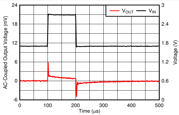
V_{\text{OUT}} = 1.2\text{ V} , I_{\text{OUT}} = 100\text{ mA} , slew rate = 1\text{ V}/\mu\text{s} , T_J = 150^\circ\text{C}
