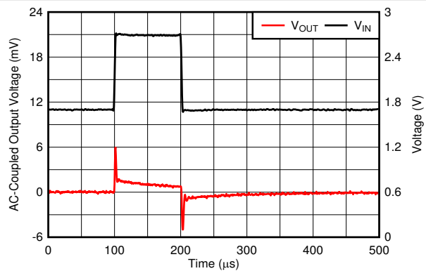
Figure 6-31. Line Transient
