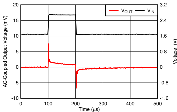
V_{\text{OUT}} = 1.2\text{ V} , I_{\text{OUT}} = 300\text{ mA} , slew rate = 1\text{ V}/\mu\text{s} , T_J = -40^\circ\text{C}
