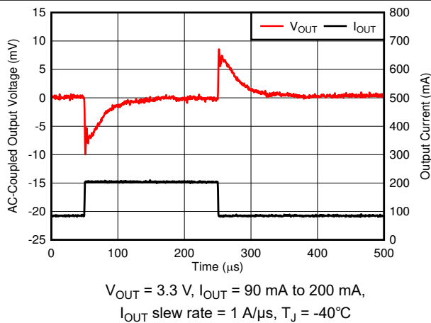
Figure 6-63. Load Transient
