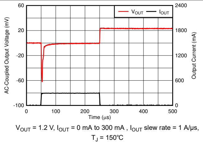
Figure 6-52. Load Transient
