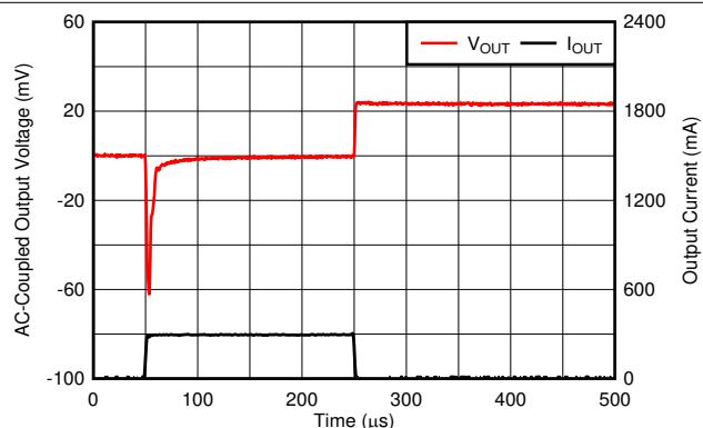
Figure 6-50. Load Transient
