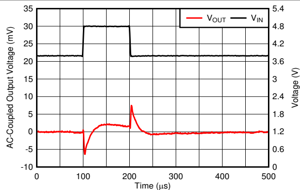
V_{\text{OUT}} = 3.3\text{ V} , I_{\text{OUT}} = 50\text{ mA} , slew rate = 1\text{ V}/\mu\text{s} , T_J = 25^\circ\text{C}
