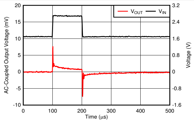
V_{\text{OUT}} = 1.2\text{ V} , I_{\text{OUT}} = 300\text{ mA} , slew rate = 1\text{ V}/\mu\text{s} , T_J = 25^\circ\text{C}
