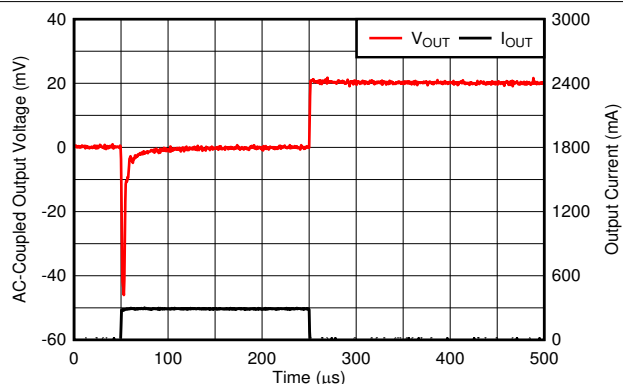
Figure 6-50. Load Transient
