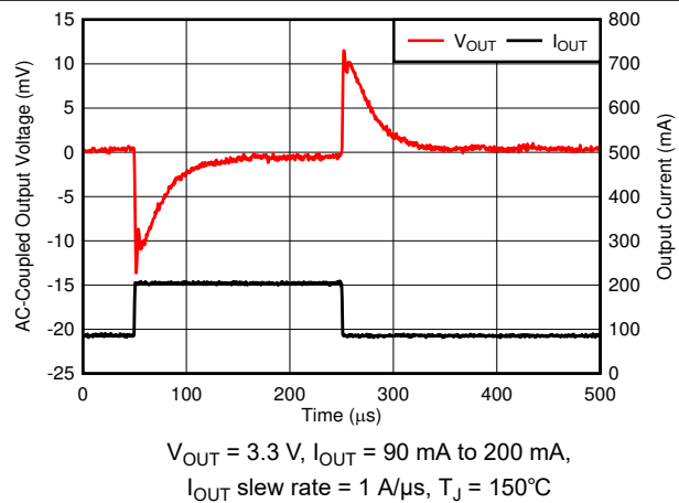
Figure 6-64. Load Transient
