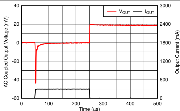
Figure 6-49. Load Transient
