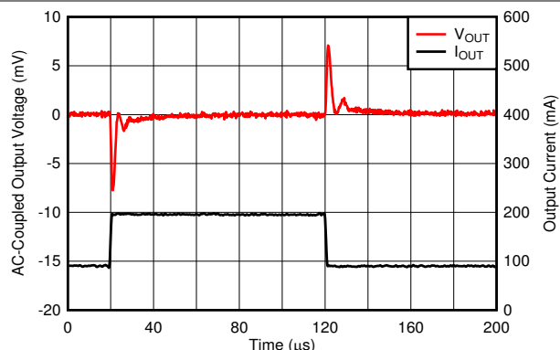
Figure 6-52. Load Transient
