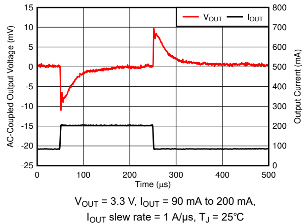
Figure 6-62. Load Transient
