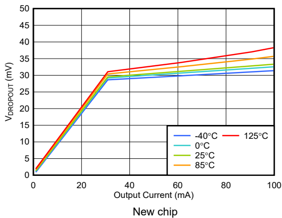
Figure 5-17. Dropout Voltage vs Output Current
