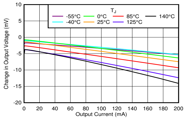
Figure 6-32. Load Regulation vs V_{IN} and Temperature
