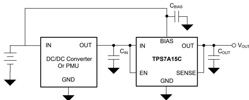
Figure 7-4. High-Efficiency Supply From a Rechargeable Battery
