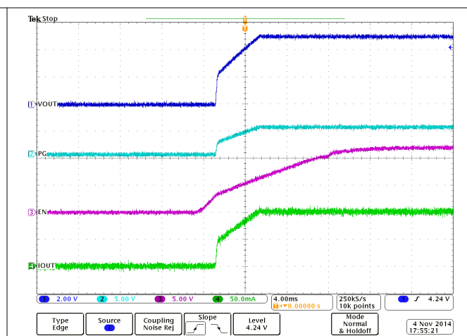
Figure 8-4. CH1 is VOUT, CH2 is PG, CH3 is EN, CH4 is Iout, VIN is 12 V Connected to EN
