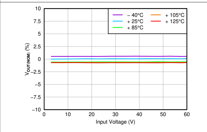
Figure 6-6. Line Regulation
