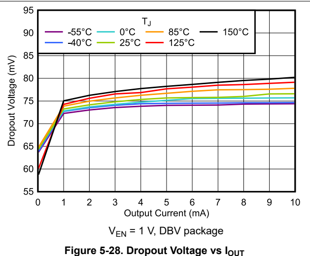
Figure 5-28. Dropout Voltage vs I_{OUT}
