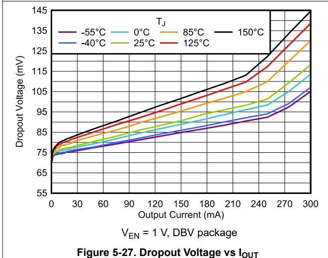
Figure 5-27. Dropout Voltage vs I_{OUT}
