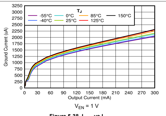
Figure 5-38. I_{GND} vs I_{OUT}
