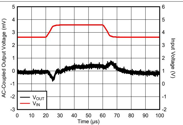
V_{EN} = V_{IN} , t_r = t_f = 5\text{ }\mu\text{s} , I_{OUT} = 1\text{ mA}
