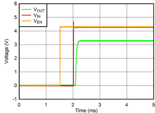
V_{IN} = 0V to 4.3V , slew rate = 1V/\mu s , I_{OUT} = 500mA Figure 5-20. Start-Up With V_{EN} Before V_{IN}
