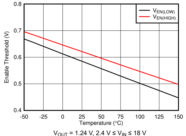
Figure 7-14. V_{EN} Thresholds vs Temperature
