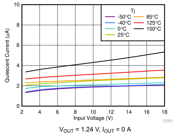
Figure 7-10. I_Q vs V_{IN}
