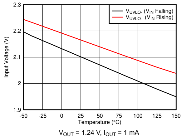
Figure 7-15. UVLO Thresholds vs Temperature
