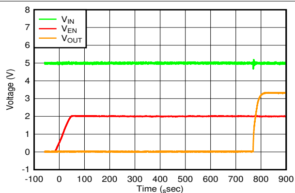
Figure 7-32. Start-Up With Enable
