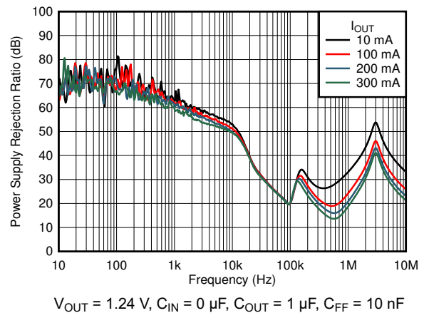
Figure 7-18. PSRR vs Frequency and I_{OUT}
