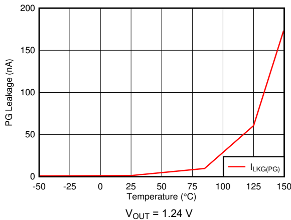
Figure 7-17. PG Leakage Current vs Temperature
