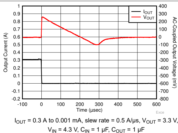
Figure 7-29. Load Transient
