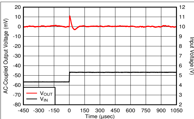
Figure 7-31. Line Transient
