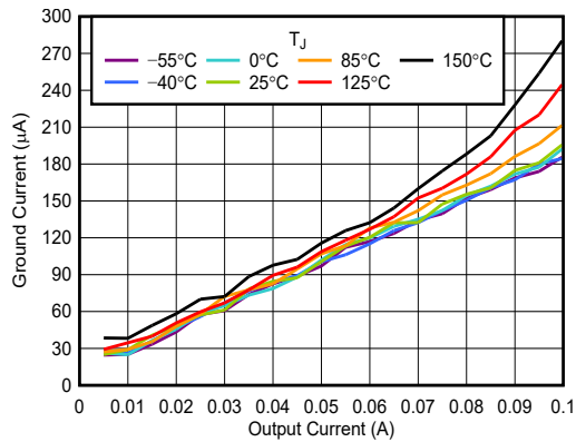
Figure 5-7. I_{GND} vs I_{OUT}
