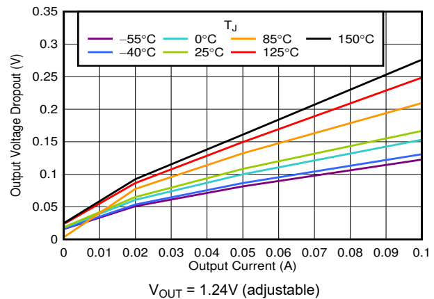
Figure 5-10. V_{DO(OUT)} vs I_{OUT}
