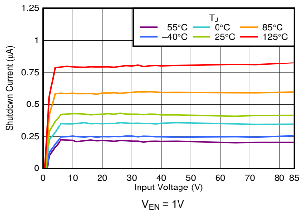
Figure 5-9. I_{SHUTDOWN} vs V_{IN}
