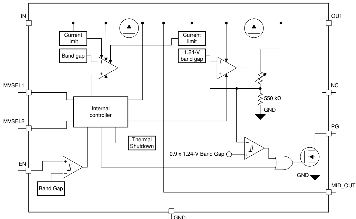
Figure 6-2. Fixed Version
