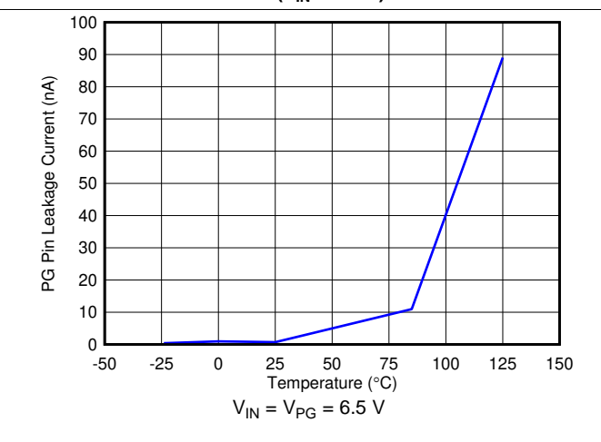
Figure 24. PG Leakage Current vs Temperature
