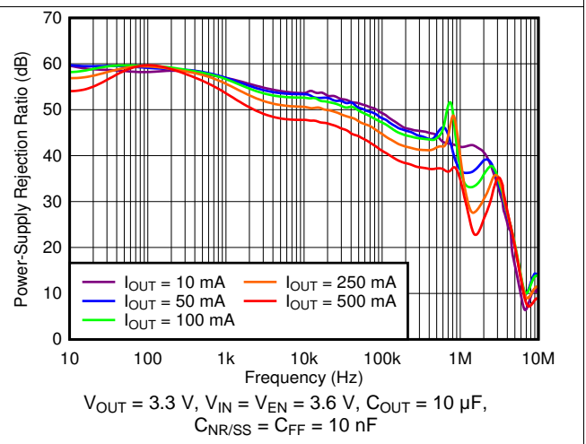
Figure 6. PSRR vs Frequency and Output Current
