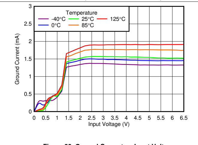
Figure 20. Ground Current vs Input Voltage
