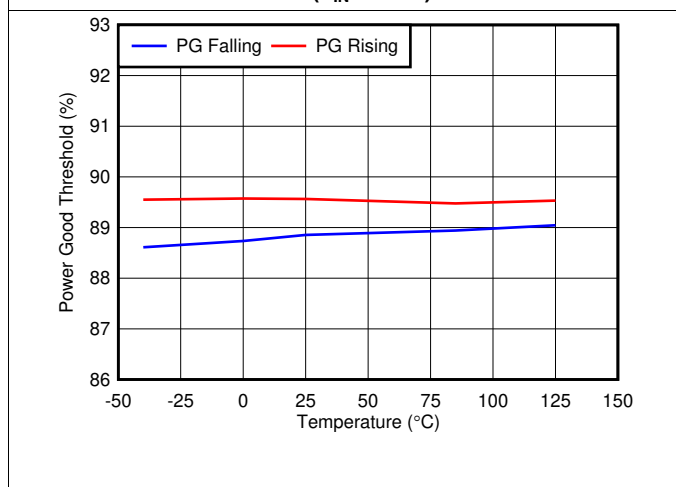
Figure 23. PG Threshold vs Temperature
