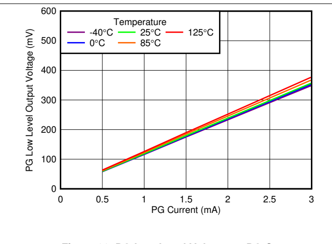
Figure 22. PG Low Level Voltage vs PG Current ( V_{IN} = 6.5\text{ V} )
