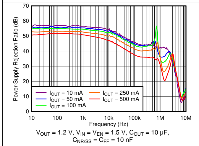
Figure 5. PSRR vs Frequency and Output Current
