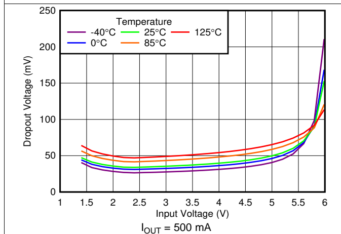
Figure 15. Dropout Voltage vs Input Voltage
