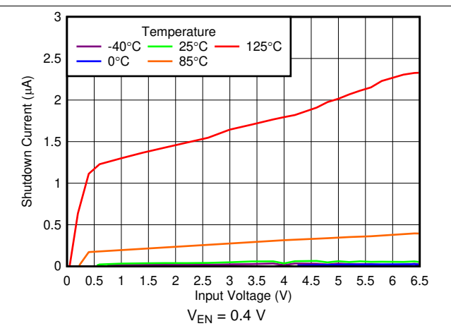
Figure 18. Shutdown Current vs Input Voltage
