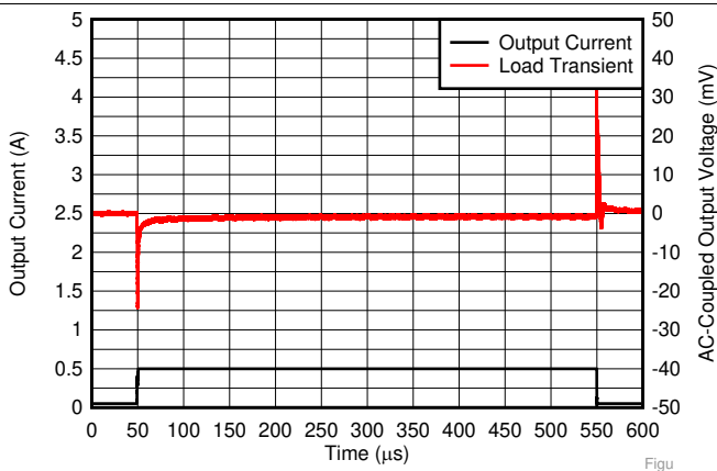
Figure 29. Load Transient Response ( V_{OUT} = 0.8\text{ V} ) V_{IN} = 1.4\text{ V} , I_{OUT} = 50\text{ mA} to 500\text{ mA} to 50\text{ mA} at 1\text{ A}/\mu\text{s} , C_{OUT} = 10\ \mu\text{F} , V_{PG} = V_{OUT}
