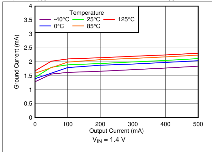
Figure 19. Ground Current vs Output Current
