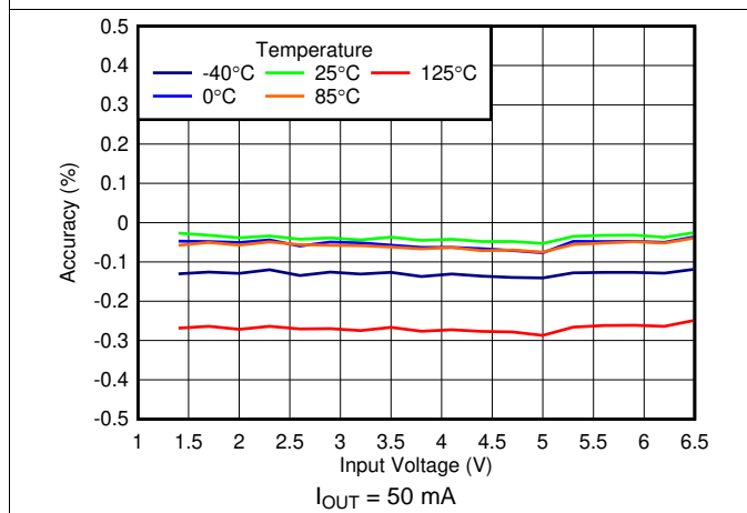
Figure 17. Line Regulation
