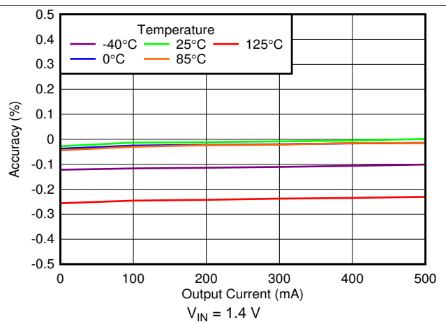
Figure 16. Load Regulation
