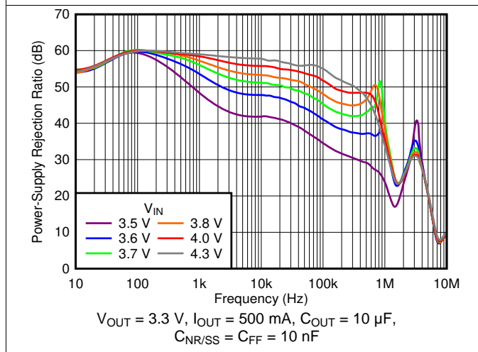
Figure 3. PSRR vs Frequency and Input Voltage
