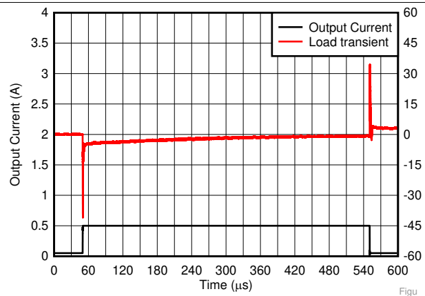
Figure 30. Load Transient Response ( V_{OUT} = 5.0\text{ V} ) V_{IN} = 5.5\text{ V} , I_{OUT} = 50\text{ mA} to 500\text{ mA} to 50\text{ mA} at 1\text{ A}/\mu\text{s} , C_{OUT} = 10\ \mu\text{F} , V_{PG} = V_{OUT}
