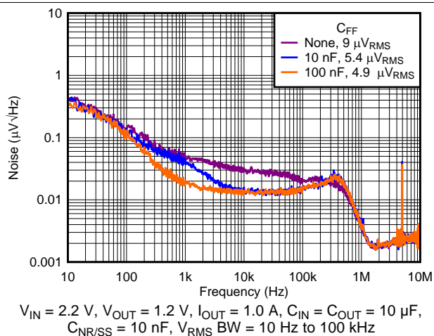
Figure 10. Spectral Noise Density vs Frequency and C_{FF}
