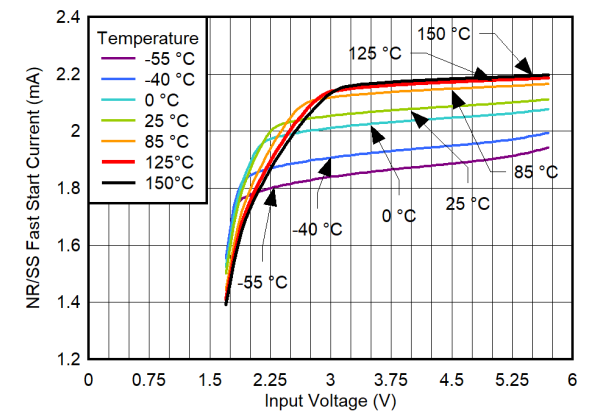
Figure 6-71. I_{NR/SS} Fast-Start vs V_{IN} and Temperature
