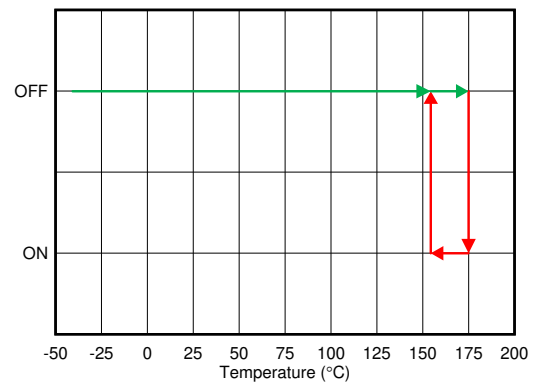
Figure 6-38. Thermal Shutdown
