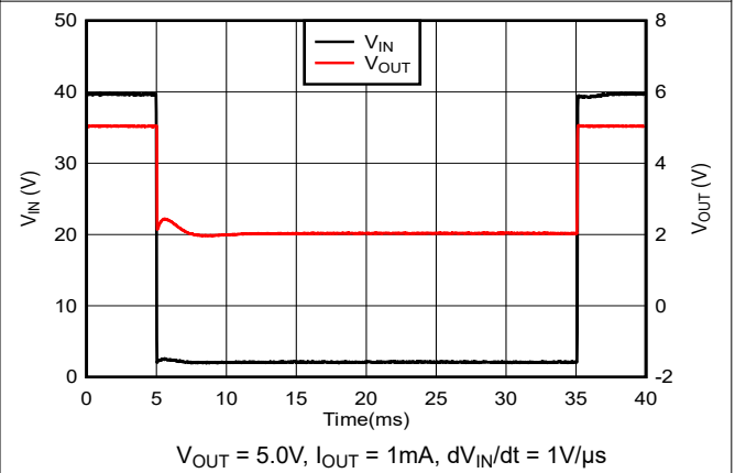
Figure 5-28. Brownout Transient (40V to 2.1V)
