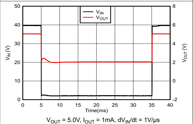
Figure 7-13. Brownout Transient (40V to 2.1V)
