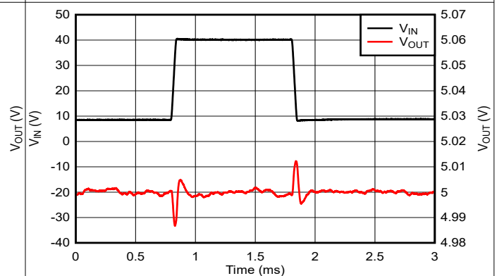
Figure 5-22. V_{IN} Line Transient (7V to 40V)
