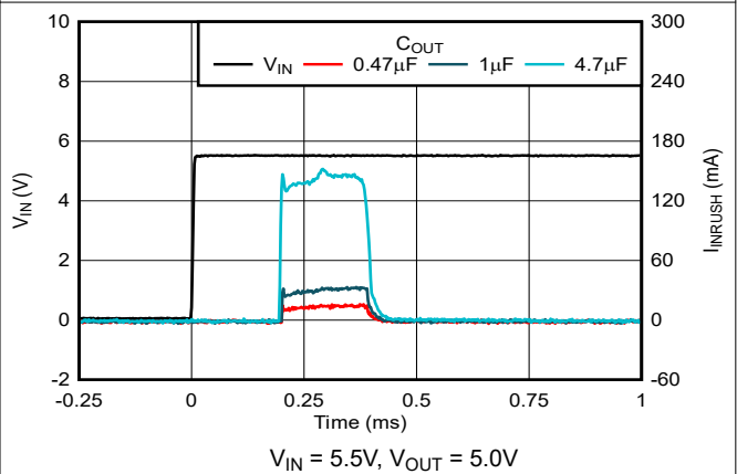
Figure 7-15. Inrush Current vs Output Capacitor
