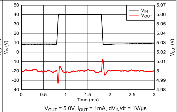
Figure 7-9. V_{IN} Line Transient (8.8V to 40V)
