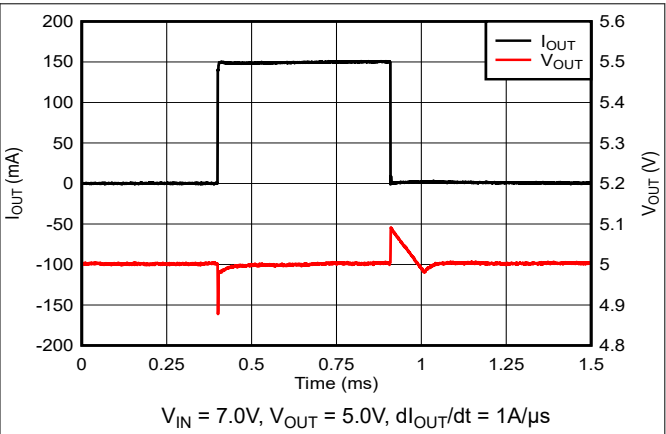
Figure 7-11. Load Transient (1mA to 150mA)
