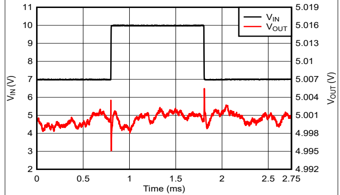
Figure 5-20. V_{IN} Line Transient (7V to 10V)
