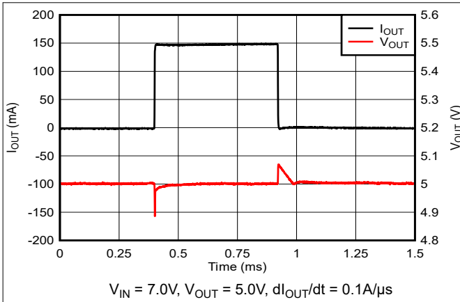
Figure 7-10. Load Transient (1mA to 150mA)
