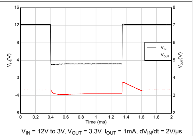
Figure 5-48. Dropout Recovery (12V to 3V)
