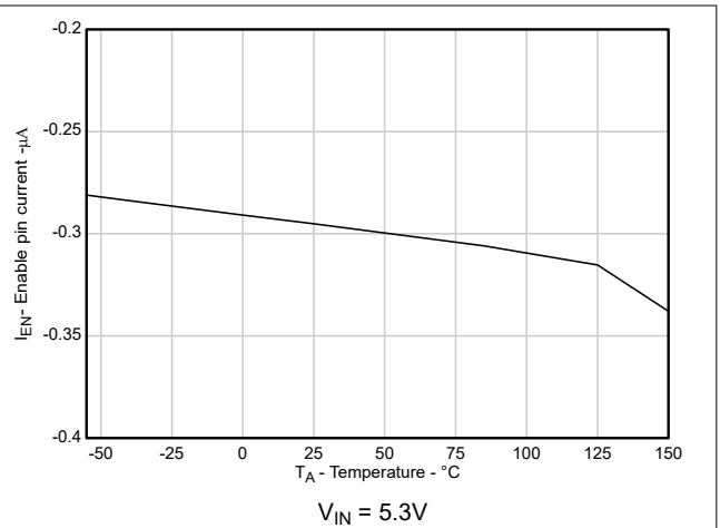
Figure 5-14. EN Leakage Current I_{EN} vs Temperature
