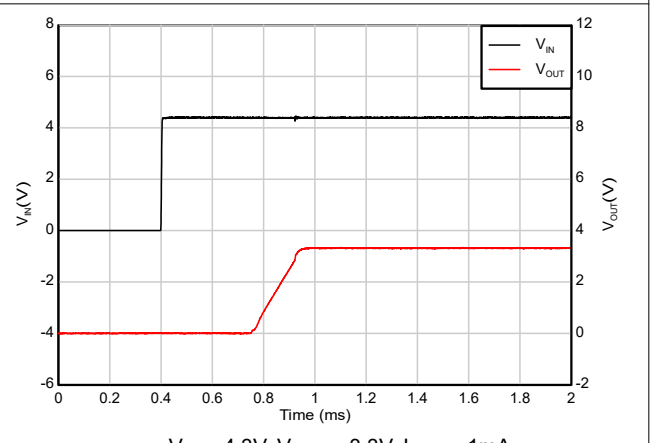
Figure 5-30. Start-up vs C_{OUT}
