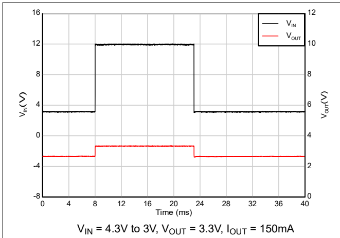
Figure 5-51. Cold-crank Recovery
