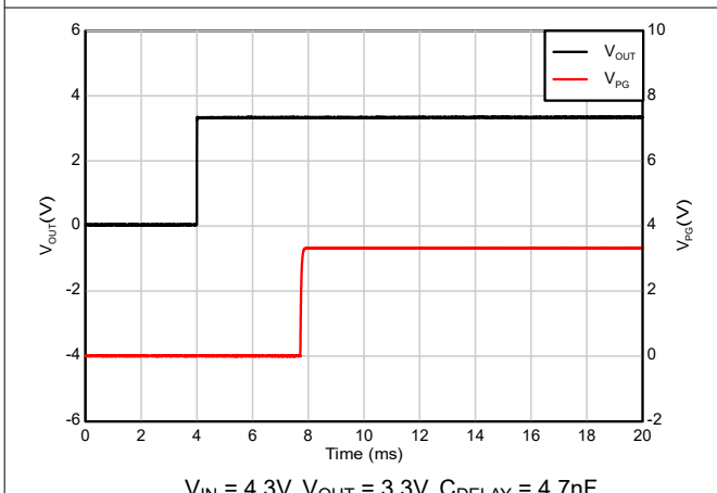
Figure 5-39. PG Delay with C_{DELAY} = 4.7\text{nF}
