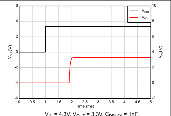
Figure 5-36. Start-up with sequencing ( V_{IN} after EN)
