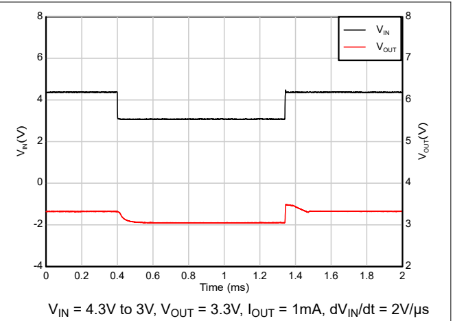
Figure 5-46. Dropout Recovery (4.3V to 3V)
