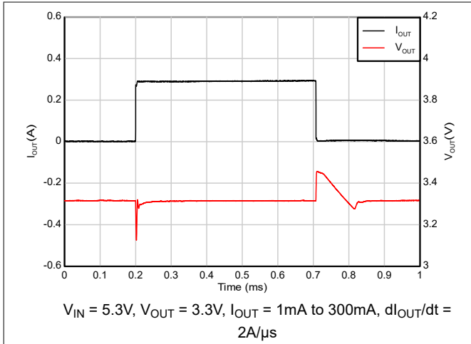
Figure 5-45. Load Transient (1mA to 300mA)
