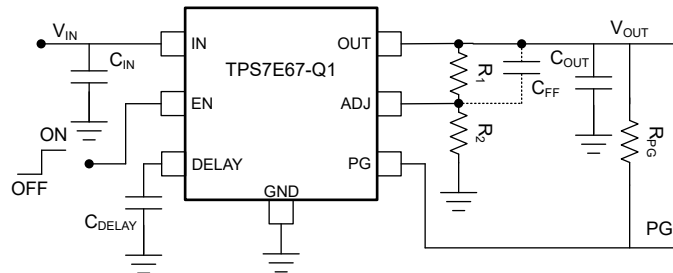
Figure 7-4. TPS7E67-Q1 Adjustable LDO Regulator Programming
