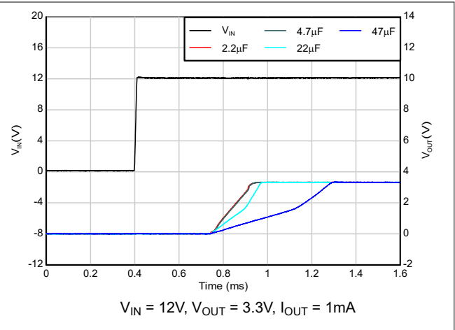
Figure 5-30. Start-up vs C_{OUT}
