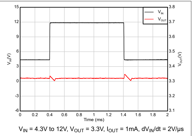
Figure 7-8. Line Transient (4.3V to 12V)
