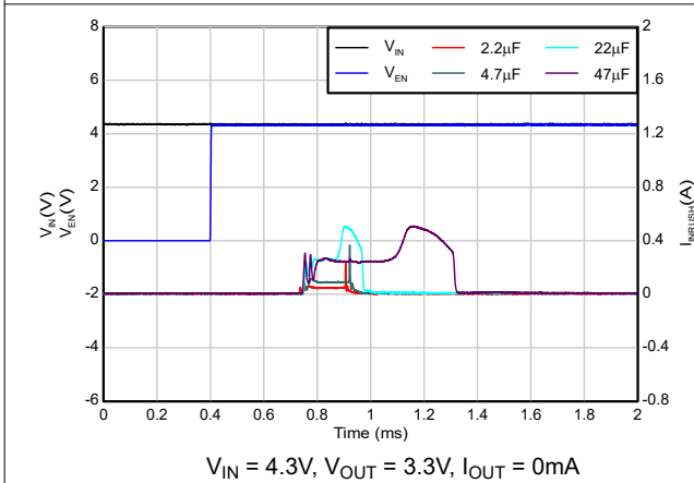
Figure 5-31. Inrush Current vs C_{OUT}
