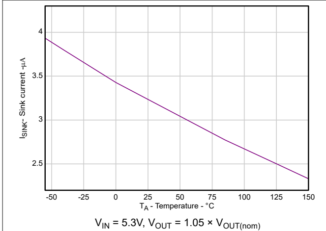
Figure 5-15. Sink Current on Output ( I_{SINK} ) vs Temperature
