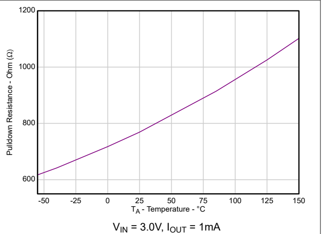
Figure 5-16. Pull-down Resistance on Output ( R_{\text{Discharge}} ) vs Temperature
