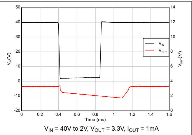
Figure 5-52. Brown-out Recovery (40V to 2V)
