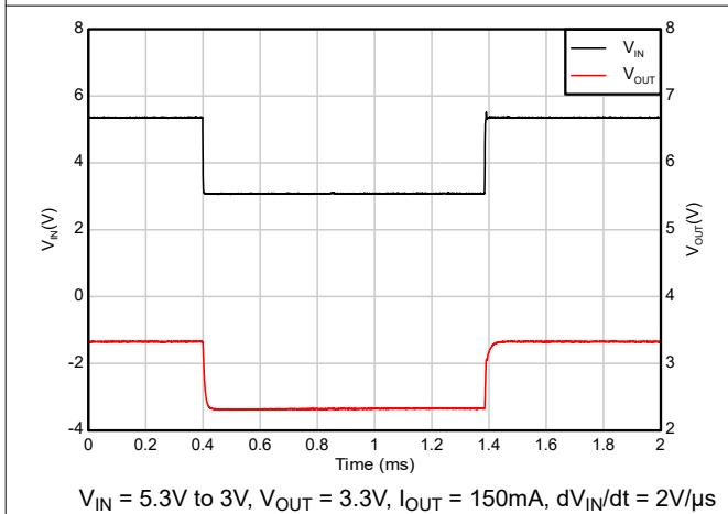
Figure 5-47. Dropout Recovery (5.3V to 3V)
