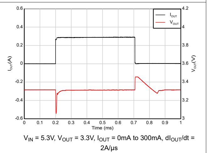
Figure 7-10. Load Transient (0mA to 300mA)
