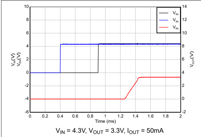
Figure 5-37. Start-up with sequencing ( V_{IN} after EN)
