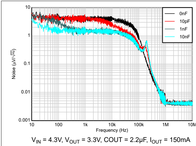
Figure 5-29. Noise vs C_{FF}
