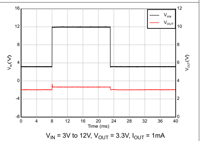
Figure 5-50. Cold-crank Recovery
