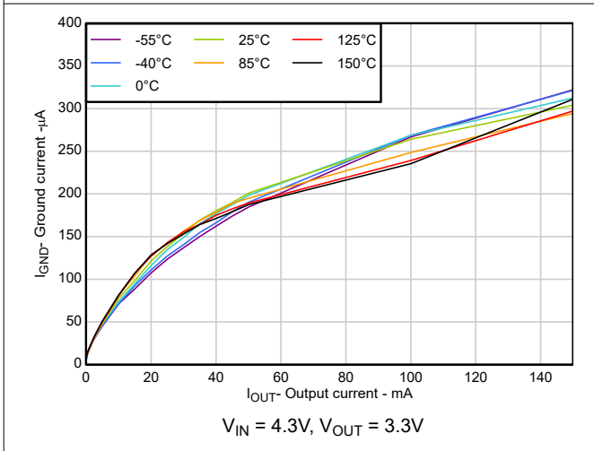
Figure 5-13. Ground Current vs Output Current
