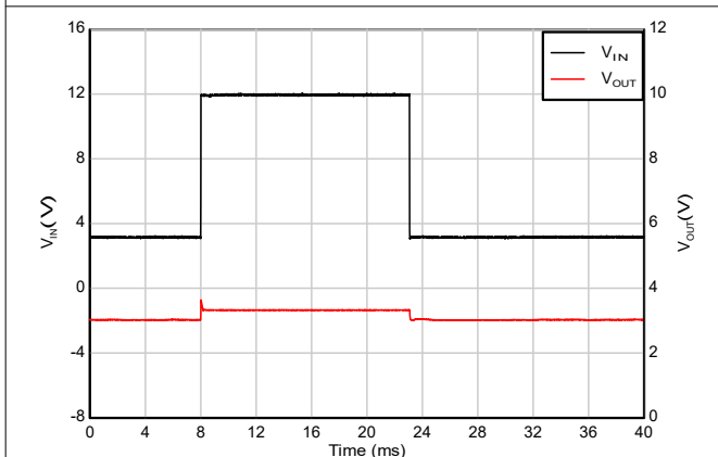
V_{IN} = 3\text{V to } 12\text{V} , V_{OUT} = 3.3\text{V} , slew rate = 2\text{V}/\mu\text{s}
