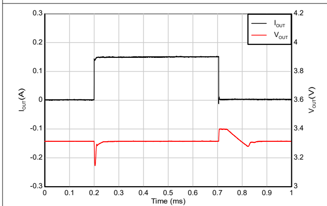
I_{OUT} = 0\text{mA to } 150\text{mA} , V_{OUT} = 3.3\text{V} , slew rate = 2\text{A}/\mu\text{s}
