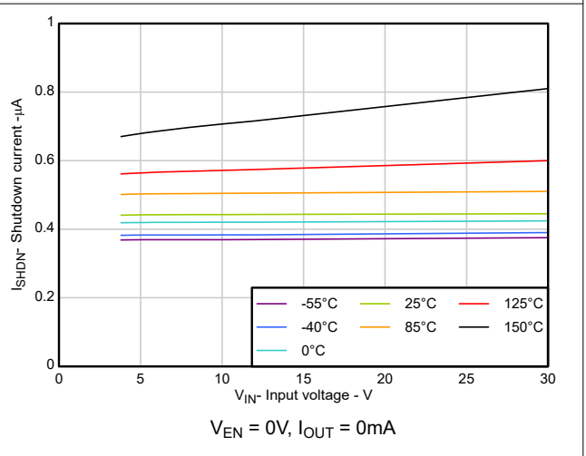
Figure 5-14. Shutdown Current vs Input Voltage
