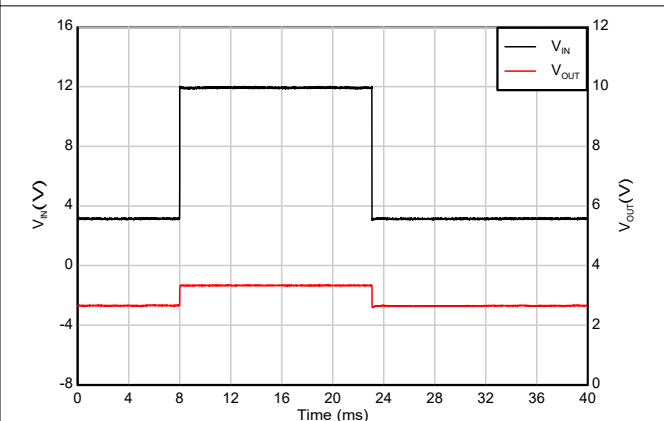
V_{IN} = 3\text{V to } 12\text{V} , V_{OUT} = 3.3\text{V} , I_{OUT} = 150\text{mA} , slew rate = 2\text{V}/\mu\text{s}
