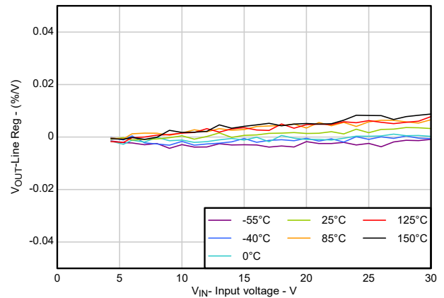
Figure 5-6. Line Regulation vs Input Voltage
