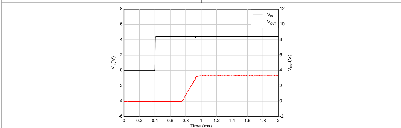
Figure 7-8. Start-up with Sequencing (EN after IN)
