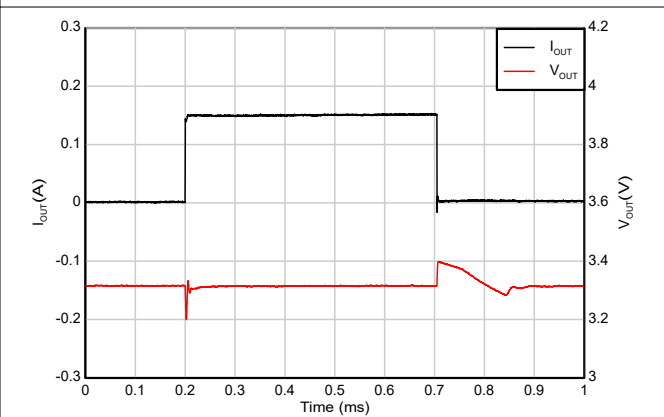
I_{OUT} = 1\text{mA to } 150\text{mA} , V_{OUT} = 3.3\text{V} , slew rate = 2\text{A}/\mu\text{s}
