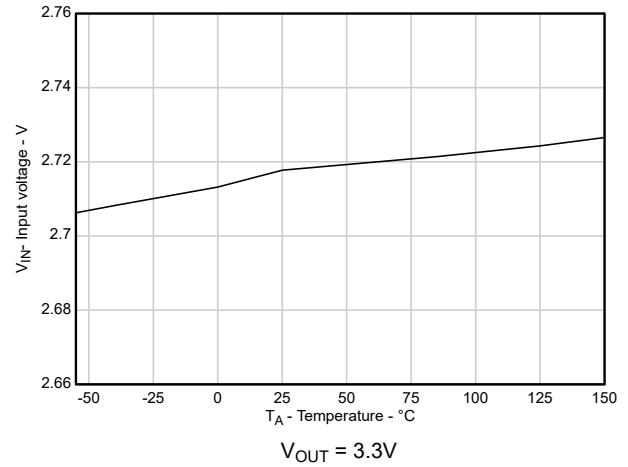
Figure 5-2. Falling Input Supply UVLO vs Temperature
