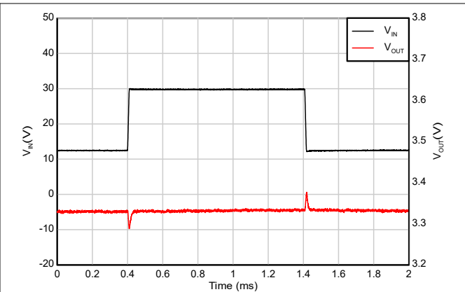
V_{IN} = 12\text{V to } 30\text{V} , V_{OUT} = 3.3\text{V} , I_{OUT} = 150\text{mA} , slew rate = 2\text{V}/\mu\text{s}
