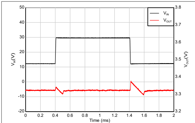
V_{IN} = 12\text{V to } 30\text{V} , V_{OUT} = 3.3\text{V} , slew rate = 2\text{V}/\mu\text{s}
