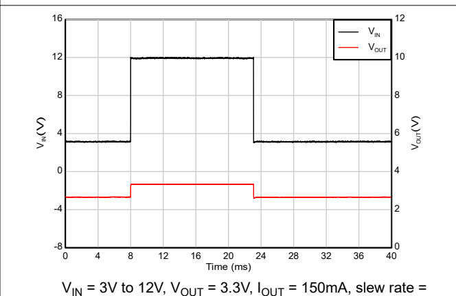
Figure 5-32. Line Transient
