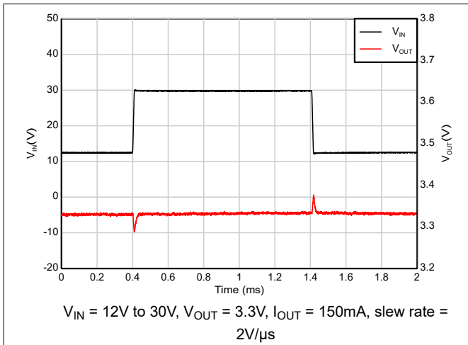
Figure 7-6. Line Transient
