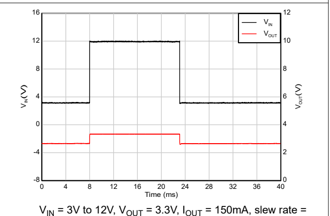
Figure 5-32. Line Transient
