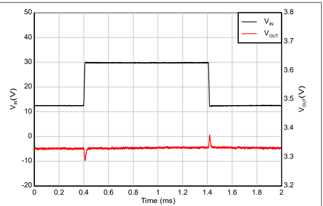
Figure 5-32. Line Transient
