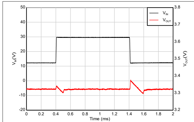
Figure 5-31. Line Transient
