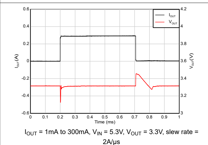
Figure 5-36. Load Transient
