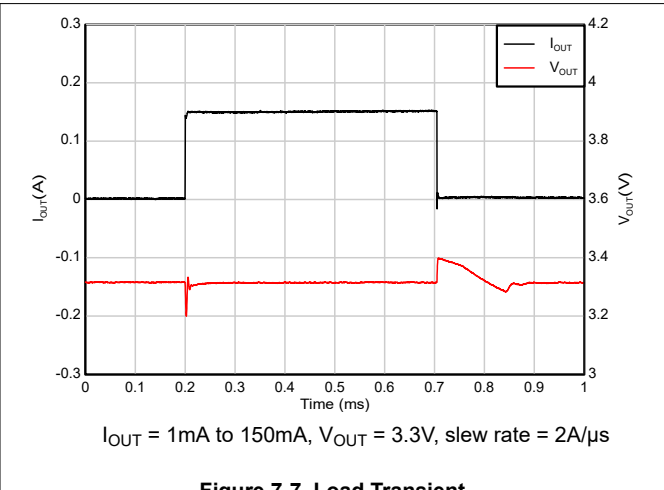
Figure 7-7. Load Transient
