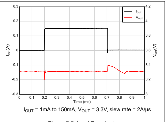
Figure 7-7. Load Transient
