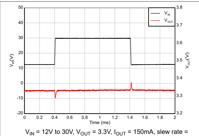
Figure 5-32. Line Transient
