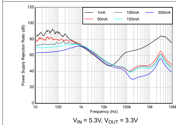
Figure 5-21. Ripple Rejection vs Frequency, Output Current
