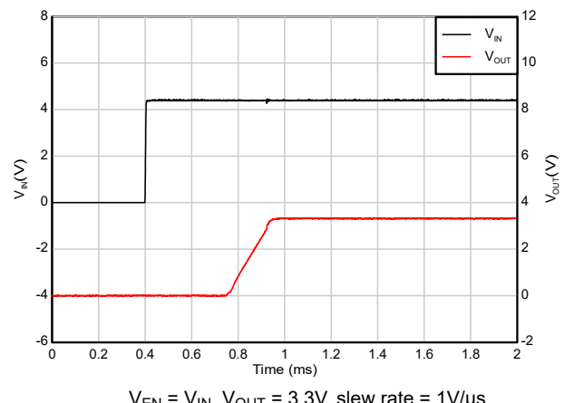
Figure 5-50. Start-up with IN & EN Tied Together
