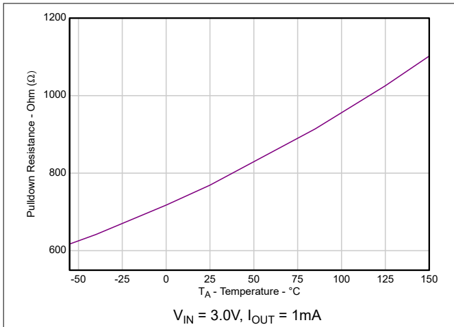
Figure 5-17. Pull-down Resistance on Output ( R_{\text{Discharge}} ) vs Temperature
