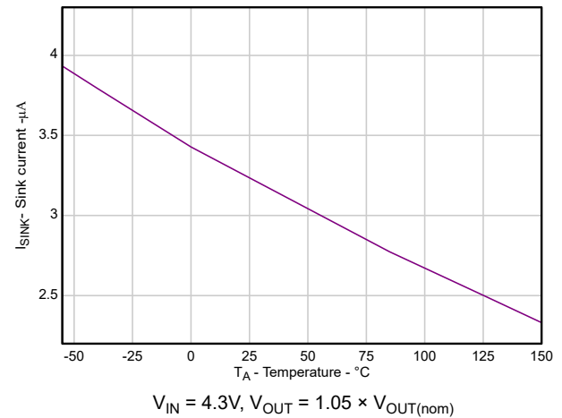
Figure 5-16. Sink Current on Output ( I_{SINK} ) vs Temperature
