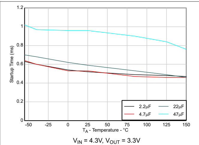
Figure 5-18. Start-up Time vs C_{\text{OUT}}
