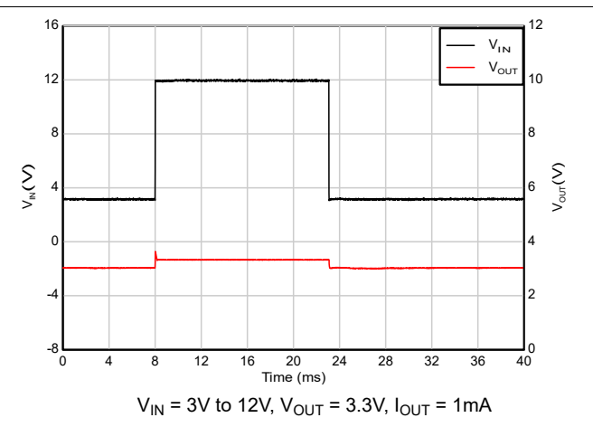
Figure 5-48. Cold-crank Recovery
