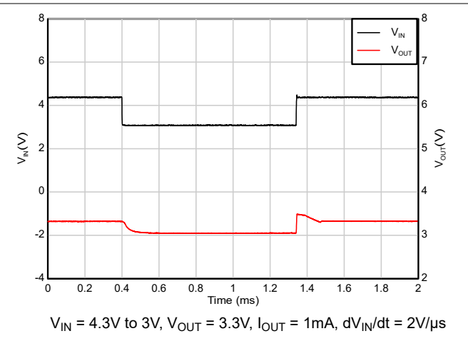
Figure 5-44. Dropout Recovery (4.3V to 3V)
