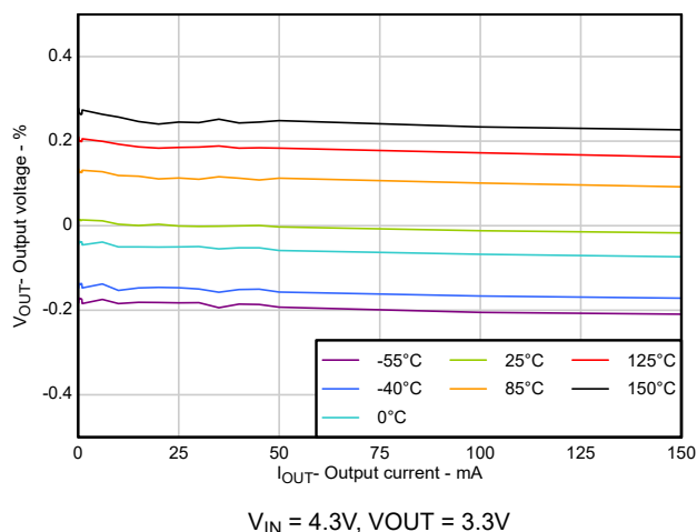
Figure 2-1. V_{OUT} Accuracy vs I_{OUT}
