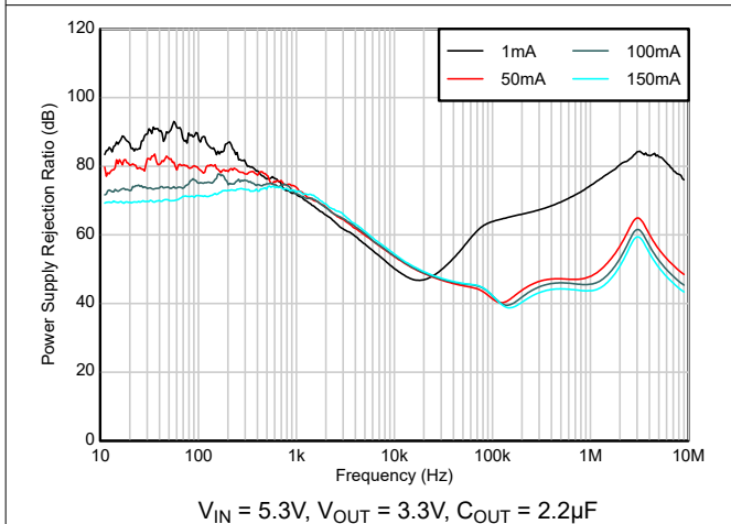
Figure 5-19. PSRR vs I_{\text{OUT}}
