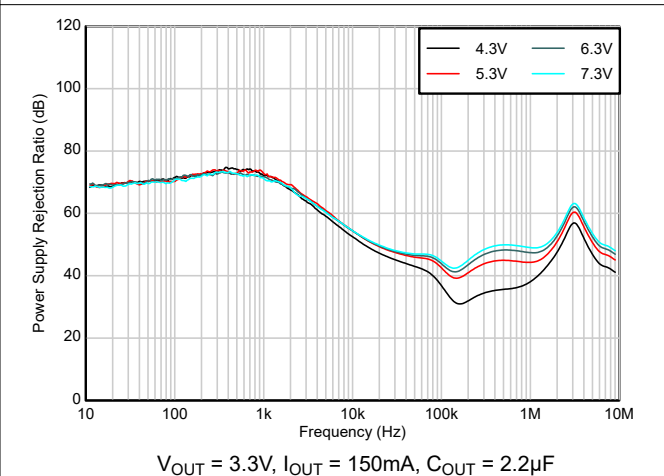
Figure 5-20. PSRR vs V_{\text{IN}}
