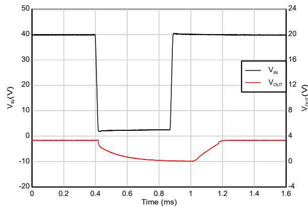
Figure 5-51. Cold-crank Recovery
