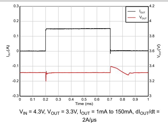
Figure 7-14. Load Transient (1mA to 150mA)
