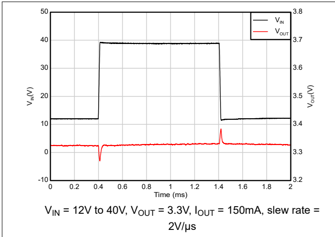
Figure 7-6. Line Transient
