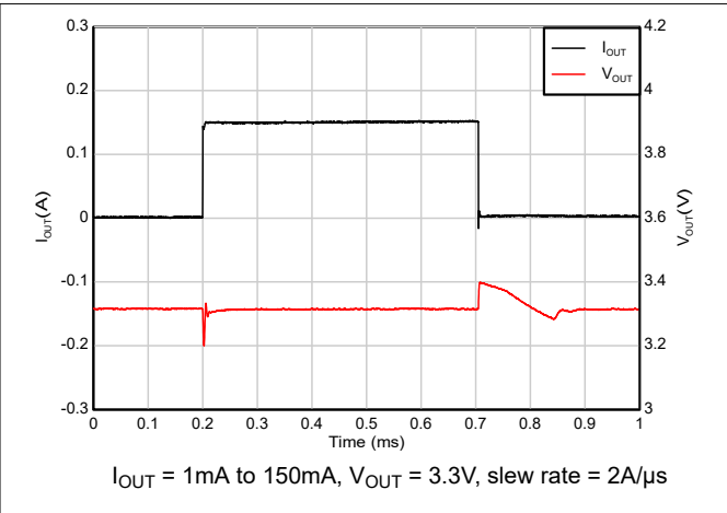
Figure 7-7. Load Transient
