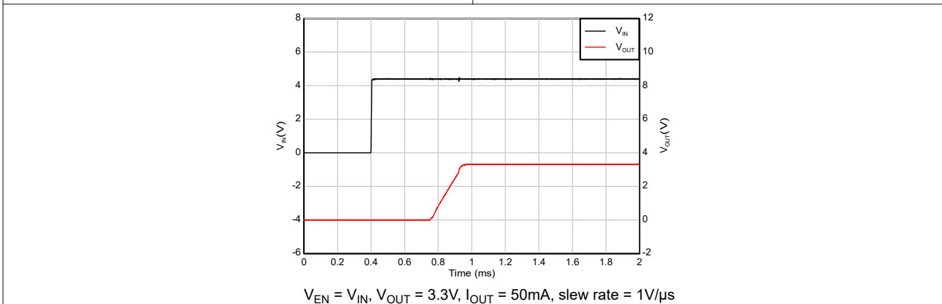
Figure 7-10. Start-up With IN and EN Tied Together
