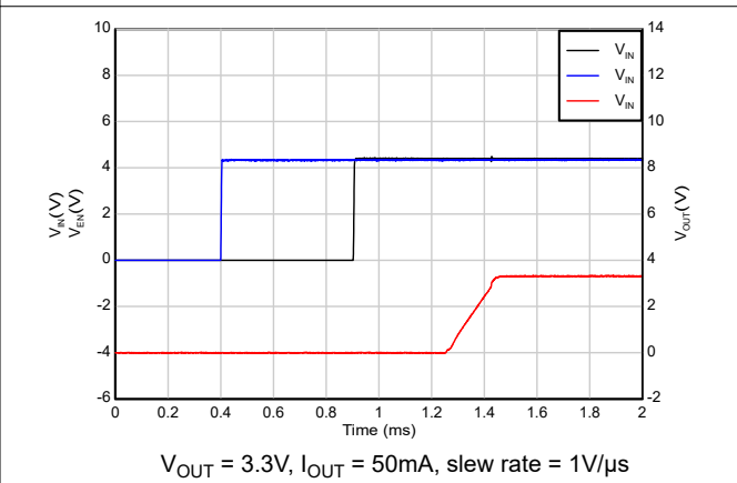
Figure 7-9. Start-up With Sequencing (IN after EN)
