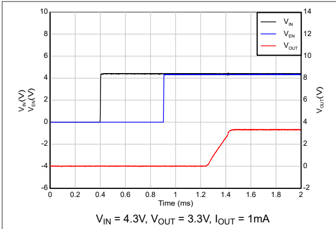
Figure 5-33. Start-up with sequencing (EN after V_{IN} )
