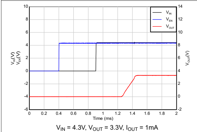
Figure 5-35. Start-up with sequencing ( V_{IN} after EN)
