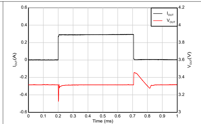
V_{IN} = 5.3\text{V} , V_{OUT} = 3.3\text{V} , I_{OUT} = 1\text{mA} to 300\text{mA} , dI_{OUT}/dt = 2\text{A}/\mu\text{s}
