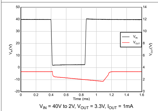
Figure 5-49. Brown-out Recovery (40V to 2V)
