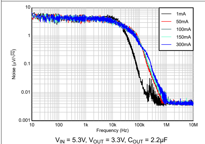
Figure 5-23. Noise vs I_{OUT}
