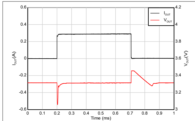
V_{IN} = 5.3\text{V} , V_{OUT} = 3.3\text{V} , I_{OUT} = 0\text{mA} to 300\text{mA} , dI_{OUT}/dt = 2\text{A}/\mu\text{s}
