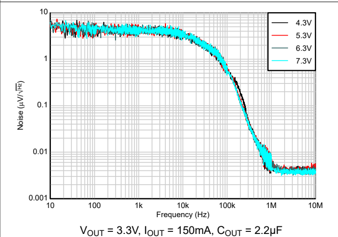
Figure 5-24. Noise vs V_{IN}
