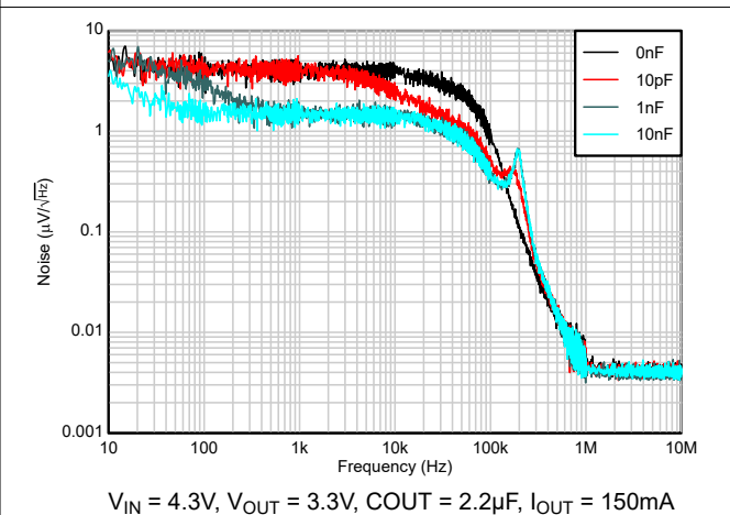
Figure 5-26. Noise vs C_{FF}
