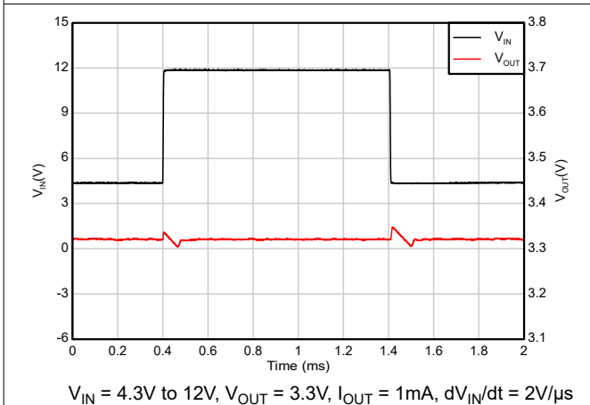
Figure 5-37. Line Transient (4.3V to 12V)
