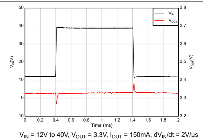
Figure 5-40. Line Transient (12V to 40V)
