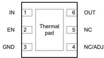
Figure 4-1. DRV Package (Fixed/ADJ), 6-Pin WSON (Top View)
