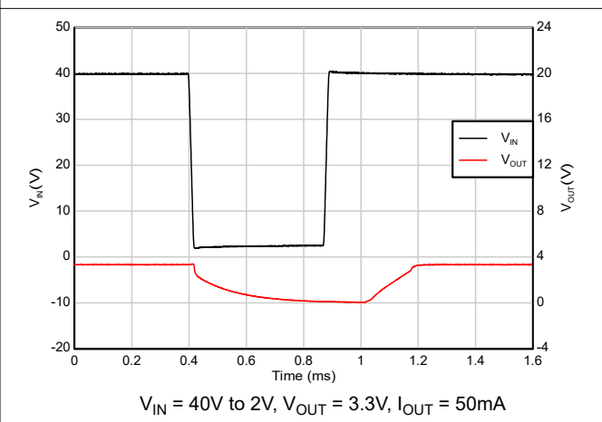
Figure 5-50. Brown-out Recovery (40V to 2V)
