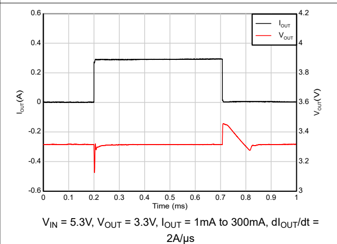
Figure 5-42. Load Transient (1mA to 300mA)
