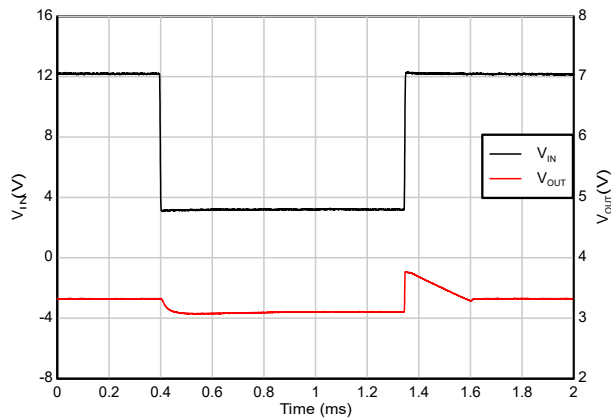
Figure 5-45. Dropout Recovery (12V to 3V)
