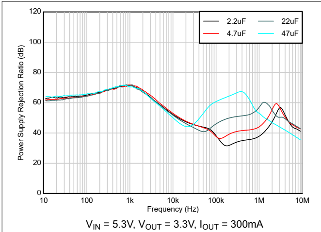
Figure 5-21. PSRR vs C_{OUT}
