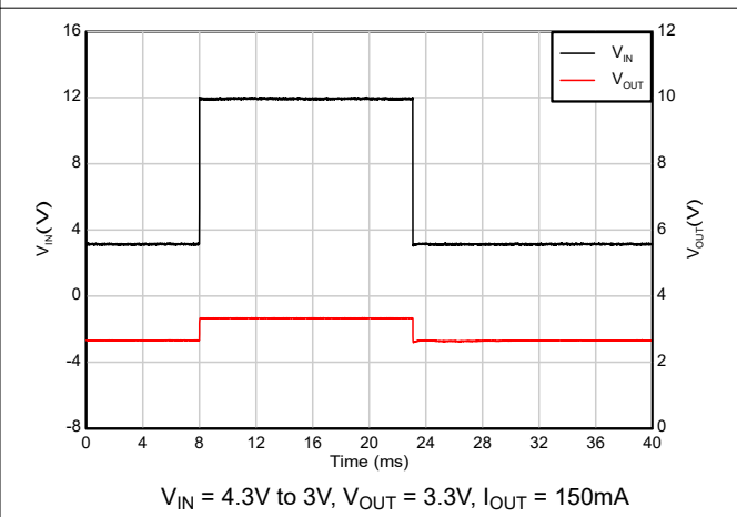
Figure 5-48. Cold-crank Recovery
