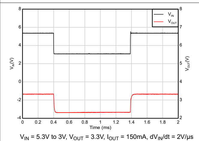
Figure 5-44. Dropout Recovery (5.3V to 3V)
