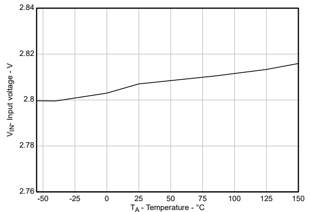
Figure 5-18. UVLO Rising Threshold ( V_{\text{UVLO+}} ) vs Temperature
