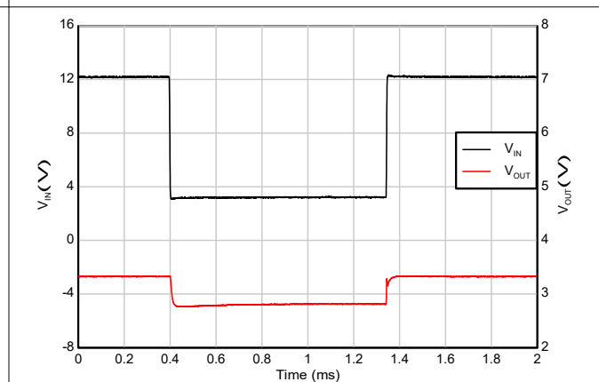
V_{IN} = 12\text{V} to 3\text{V} , V_{OUT} = 3.3\text{V} , I_{OUT} = 100\text{mA} , dV_{IN}/dt = 2\text{V}/\mu\text{s}
