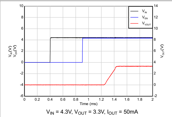
Figure 5-34. Start-up with sequencing (EN after V_{IN} )
