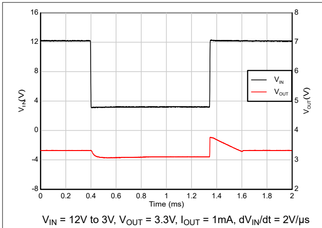
Figure 5-45. Dropout Recovery (12V to 3V)
