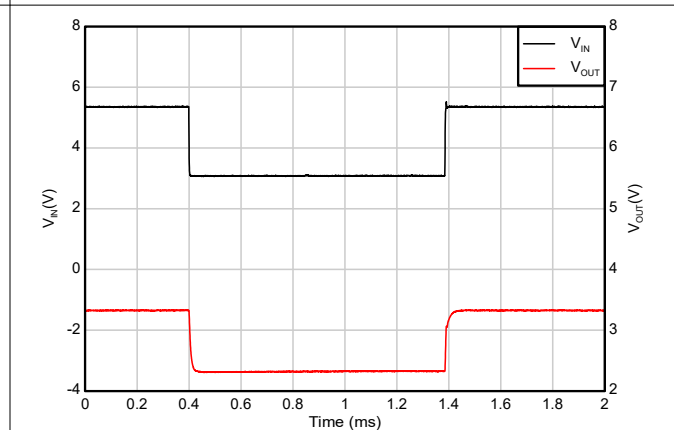
V_{IN} = 5.3\text{V} to 3\text{V} , V_{OUT} = 3.3\text{V} , I_{OUT} = 150\text{mA} , dV_{IN}/dt = 2\text{V}/\mu\text{s}
