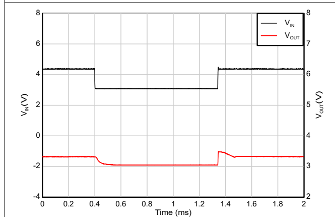
V_{IN} = 4.3\text{V} to 3\text{V} , V_{OUT} = 3.3\text{V} , I_{OUT} = 1\text{mA} , dV_{IN}/dt = 2\text{V}/\mu\text{s}
