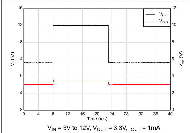
Figure 5-47. Cold-crank Recovery
