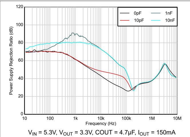
Figure 5-22. PSRR vs C_{FF}
