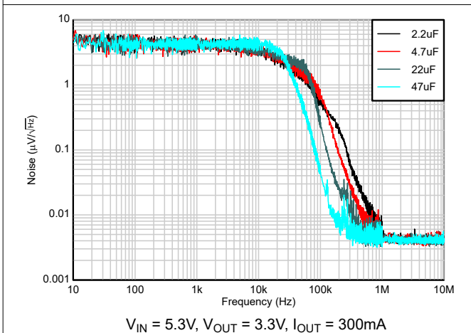
Figure 5-25. Noise vs C_{OUT}
