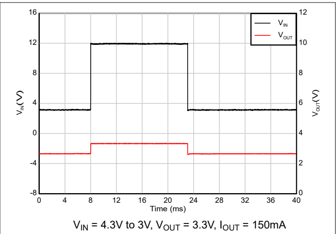
Figure 5-46. Cold-crank Recovery
