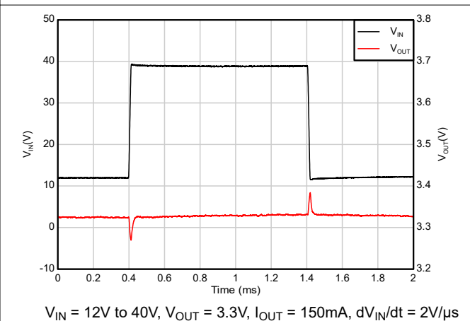
Figure 5-38. Line Transient (12V to 40V)
