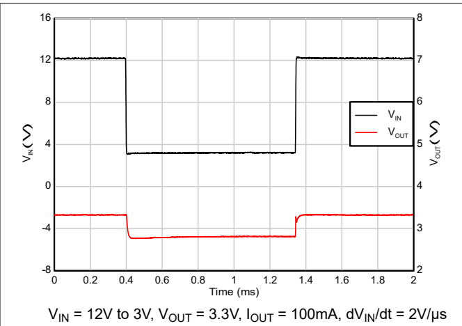
Figure 5-46. Dropout Recovery (12V to 3V)
