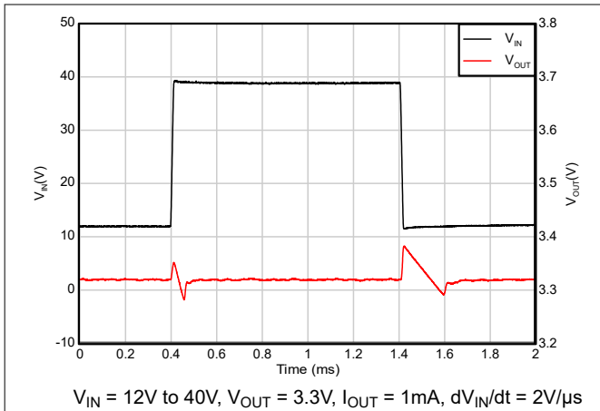
Figure 5-39. Line Transient (12V to 40V)
