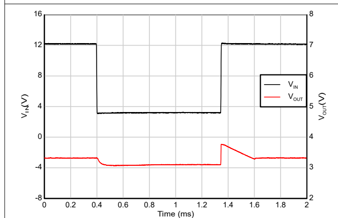
V_{IN} = 12\text{V} to 3\text{V} , V_{OUT} = 3.3\text{V} , I_{OUT} = 1\text{mA} , dV_{IN}/dt = 2\text{V}/\mu\text{s}
