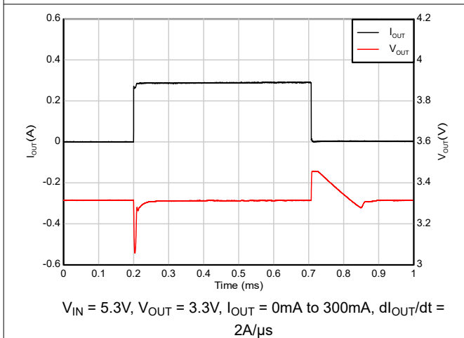
Figure 5-41. Load Transient (0mA to 300mA)
