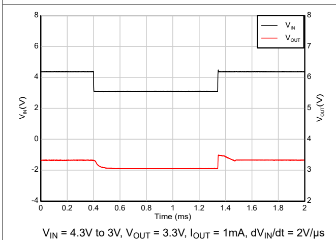
Figure 5-43. Dropout Recovery (4.3V to 3V)
