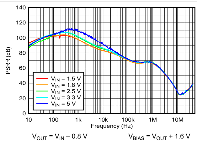
Figure 6-6. PSRR vs Frequency Across Input Voltage
