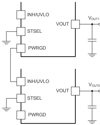
Figure 30. Sequencing Schematic
