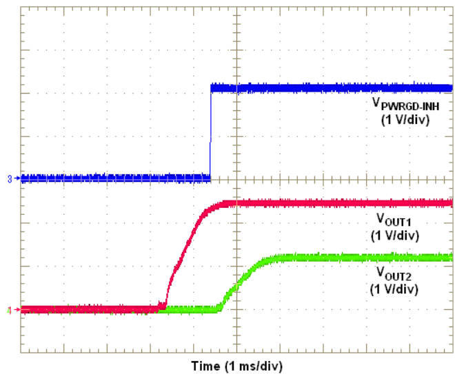
Figure 31. Sequencing Waveforms
