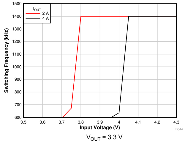
Figure 7-8. Frequency Foldback
