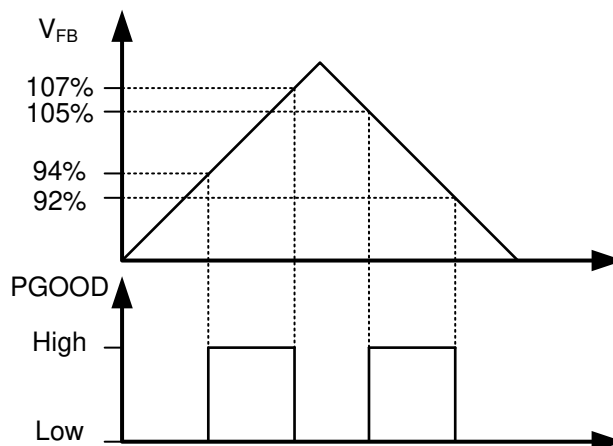
Figure 7-6. Power-good Flag
