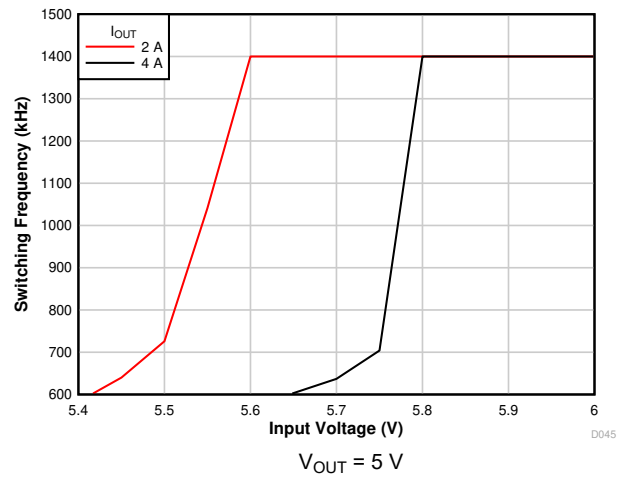
Figure 7-10. Frequency Foldback
