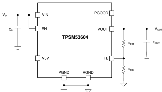
Simplified Schematic
