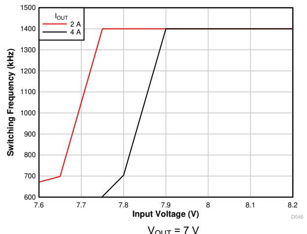
Figure 7-12. Frequency Foldback
