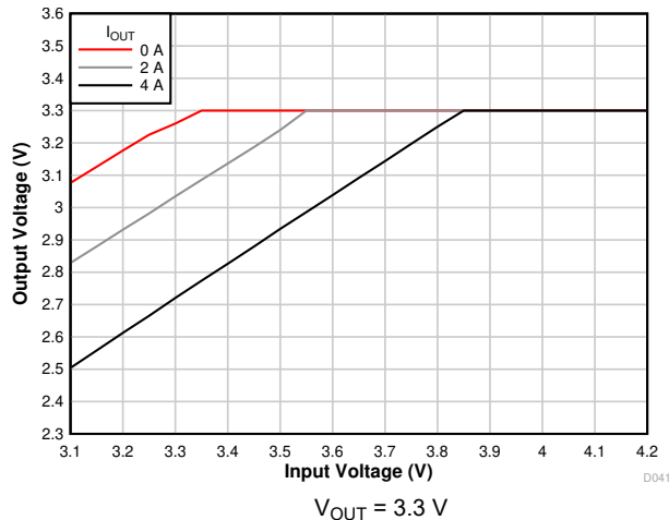
Figure 7-7. Voltage Dropout
