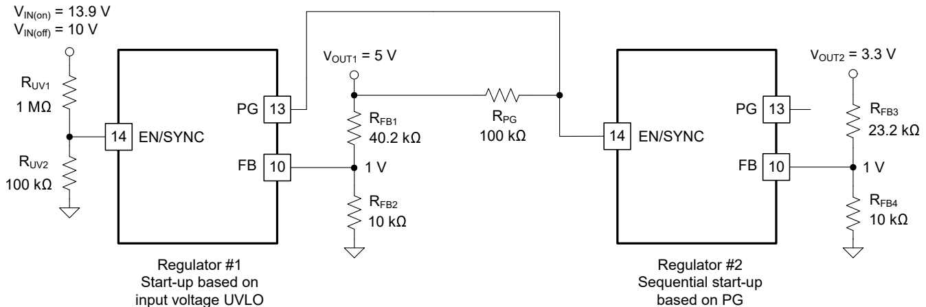
Figure 8-6. TPSM63602 Sequencing Implementation Using PG and EN/SYNC
