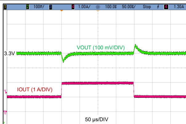
Figure 9-5. Load Transient, 1 A to 2 A, 1 A/μs
