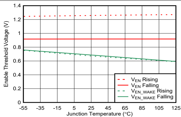
Figure 7-5. Enable Thresholds
