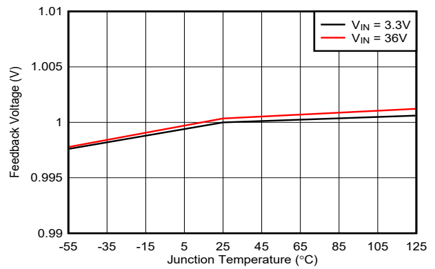
Figure 7-2. Feedback Voltage
