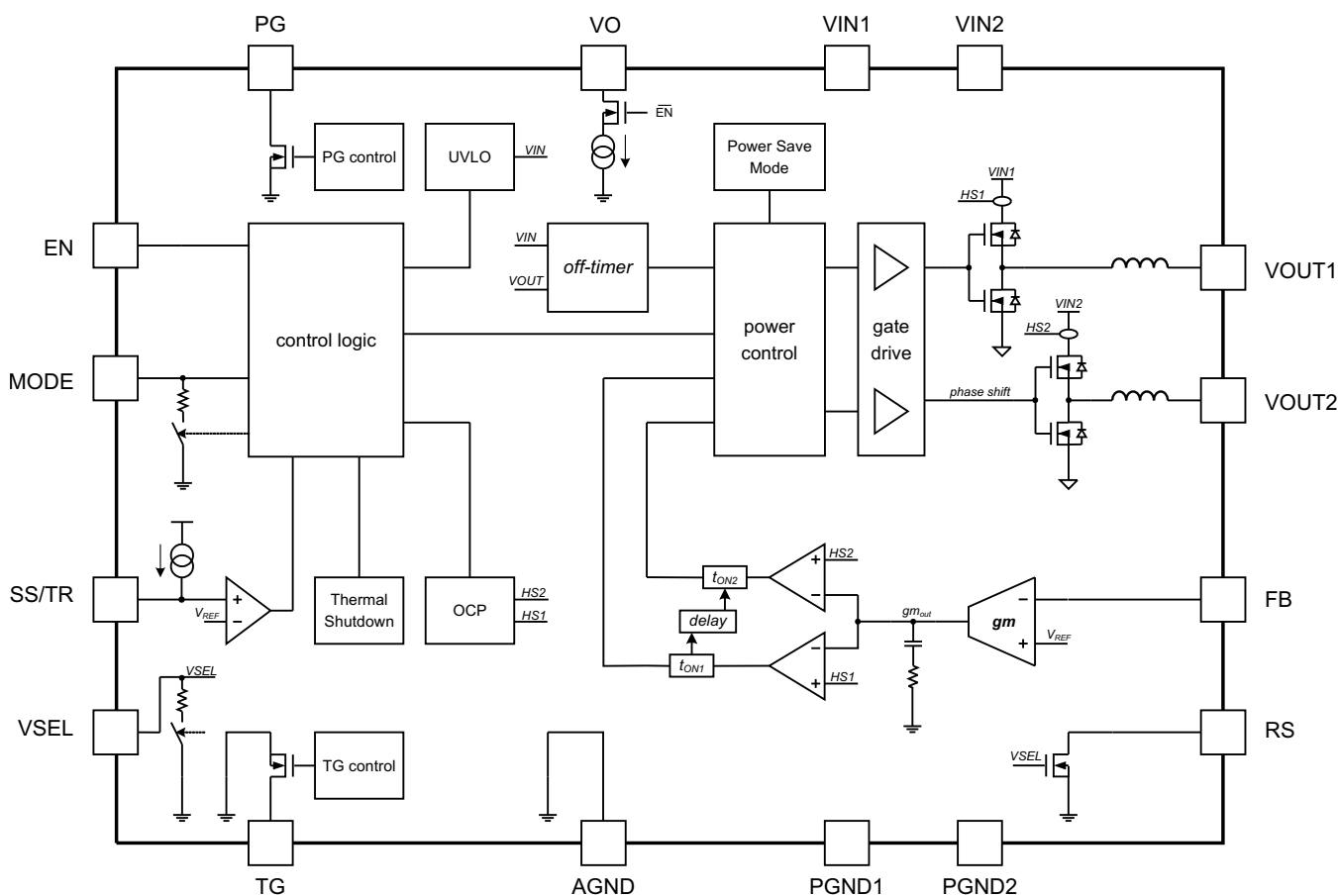
Figure 6. TPSM82480
