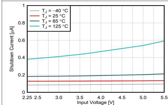
Figure 6-3. Shutdown Current
