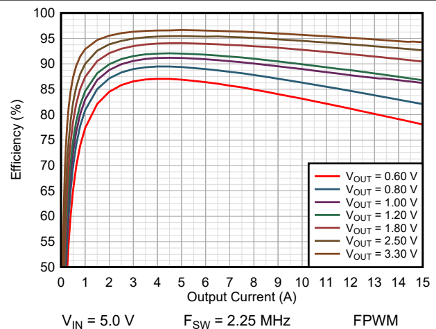
Figure 9-19. Efficiency TPSM8287A15BBH
