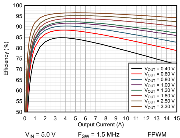
Figure 9-18. Efficiency TPSM8287A15BAH
