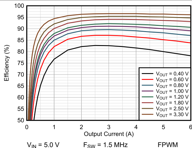
Figure 9-6. Efficiency TPSM8287A06BAS
