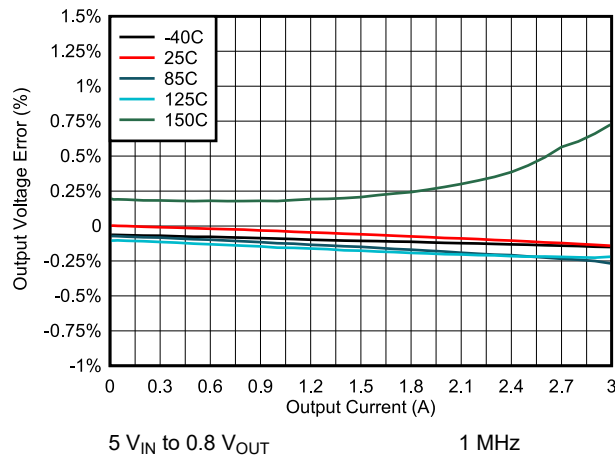
Figure 6-39. Output Voltage Error vs Load
