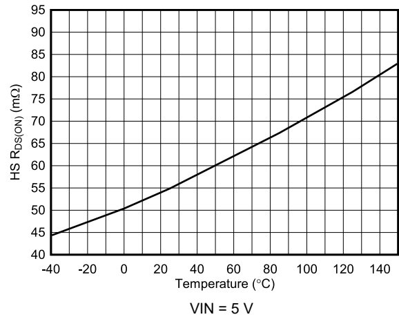
Figure 6-36. High-Side R_{DS(ON)} vs Junction Temperature
