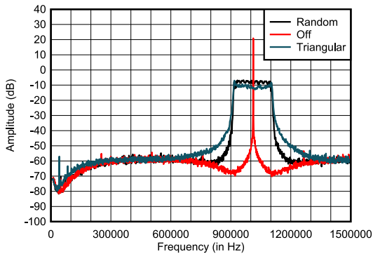
Figure 6-25. Spread Spectrum FFT - 50-Hz BW
