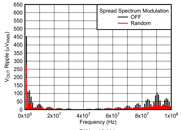
Figure 6-4. V_{OUT} Ripple FFT After the Second L-C Filter
