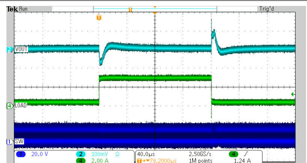
12 V to 1.8 V 1 MHz After 2nd L-C 300 mA to 3 A to 300 mA Figure 8-12. Load Transient
