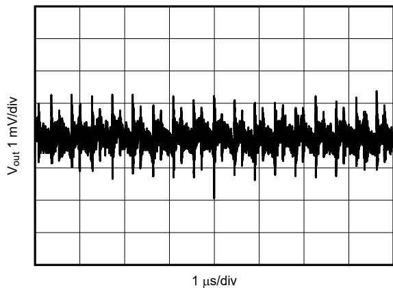
Figure 6-17. V_{OUT} Ripple After the First L-C Filter
