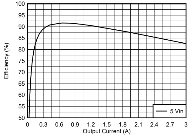
1.8 Vout 2.2 \mu H, 2.2 MHz 1st L-C Only Figure 8-8. Efficiency vs Load Current
