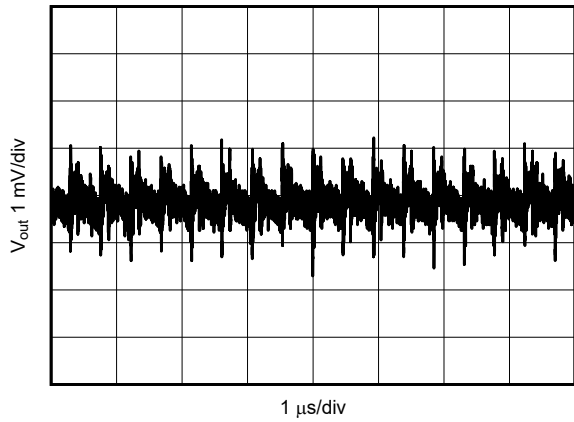
Figure 6-13. V_{OUT} Ripple After the First L-C Filter
