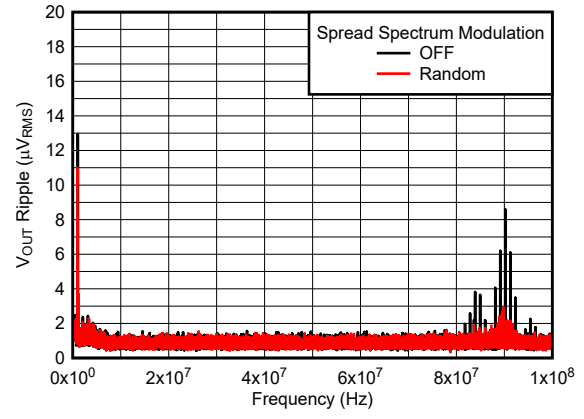
12 V to 1.8 V, 1 A 2.2 \mu\text{H} , 1 MHz First and second L-C Figure 6-8. V_{OUT} Ripple FFT After the Second L-C Filter
