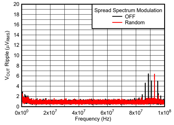
Figure 6-14. V_{OUT} Ripple FFT After the First L-C Filter
