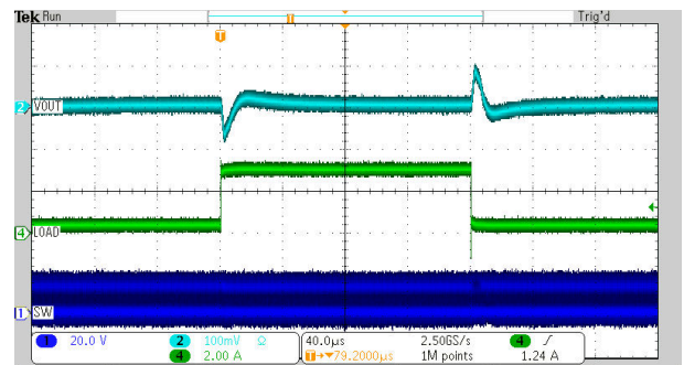
12 V to 1.8 V 1 MHz 1st L-C Only 300 mA to 3 A to 300 mA Figure 8-11. Load Transient
