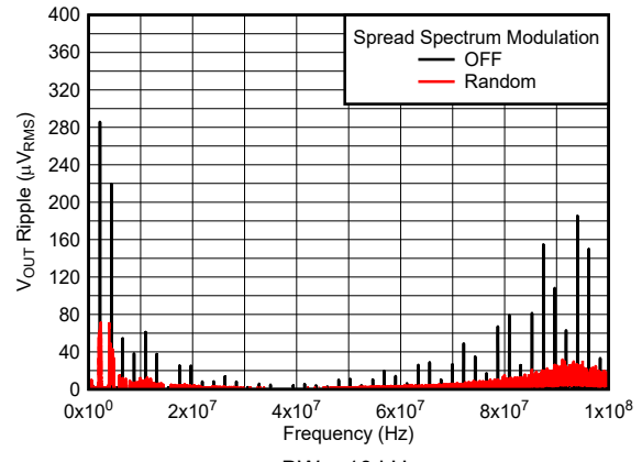
12 V to 3.3 V, 1 A 2.2 \mu\text{H} , 2.2 MHz First L-C Only Figure 6-10. V_{OUT} Ripple FFT After the First L-C Filter
