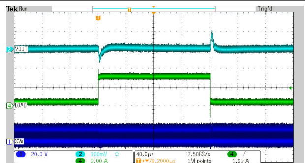
12 V to 3.3 V 2.2 MHz 1st L-C Only 300 mA to 3 A to 300 mA Figure 8-13. Load Transient
