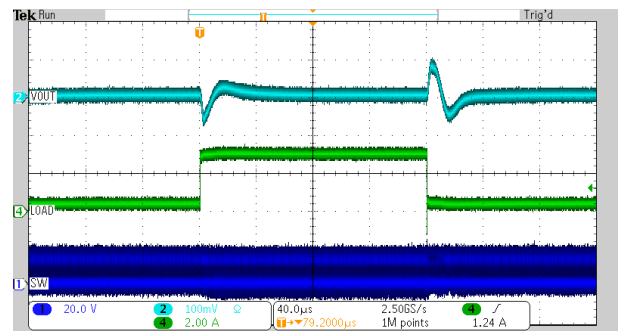
12 V to 1.2 V 1 MHz After 2nd L-C 300 mA to 3 A to 300 mA Figure 8-10. Load Transient
