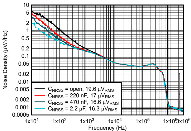
Figure 6-27. Output Noise Density vs Frequency
