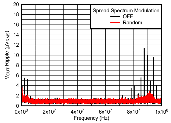
12 V to 3.3 V, 1 A 2.2 \mu\text{H} , 2.2 MHz First and second L-C Figure 6-12. V_{OUT} Ripple FFT After the Second L-C Filter
