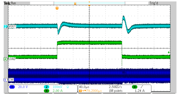
12 V to 1.2 V 1 MHz 1st L-C Only 300 mA to 3 A to 300 mA Figure 8-9. Load Transient
