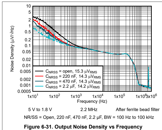
Figure 6-31. Output Noise Density vs Frequency
