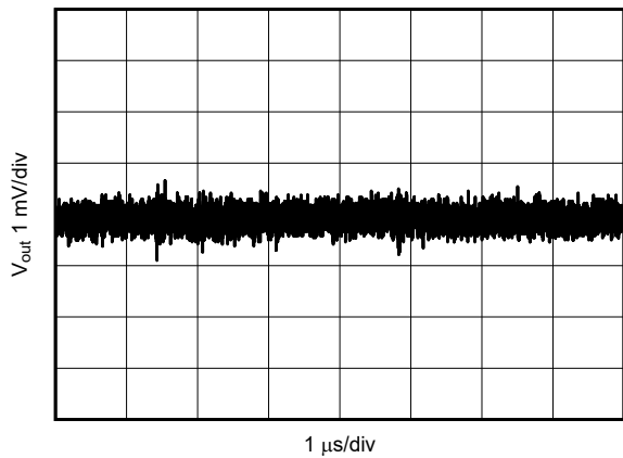
Figure 6-15. V_{OUT} Ripple after the Second L-C Filter
