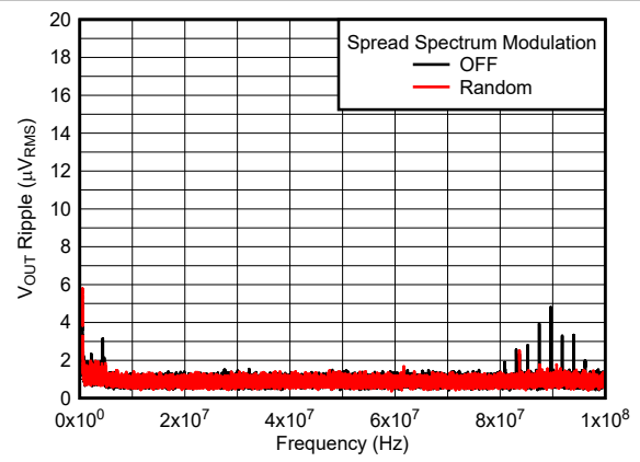
BW = 10 kHz 5 V to 3.3 V, 1 A 2.2 \mu\text{H} , 2.2 MHz First and second L-C Figure 6-24. V_{OUT} Ripple FFT After the Second L-C Filter
