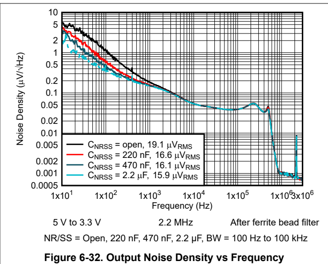
Figure 6-32. Output Noise Density vs Frequency
