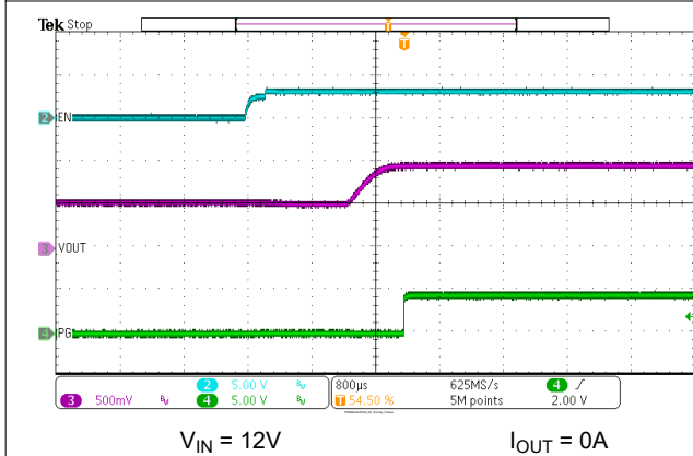
Figure 7-12. EN Start-Up – 0.5V Prebias
