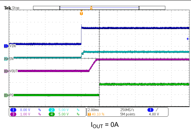
Figure 7-13. VIN Start-Up
