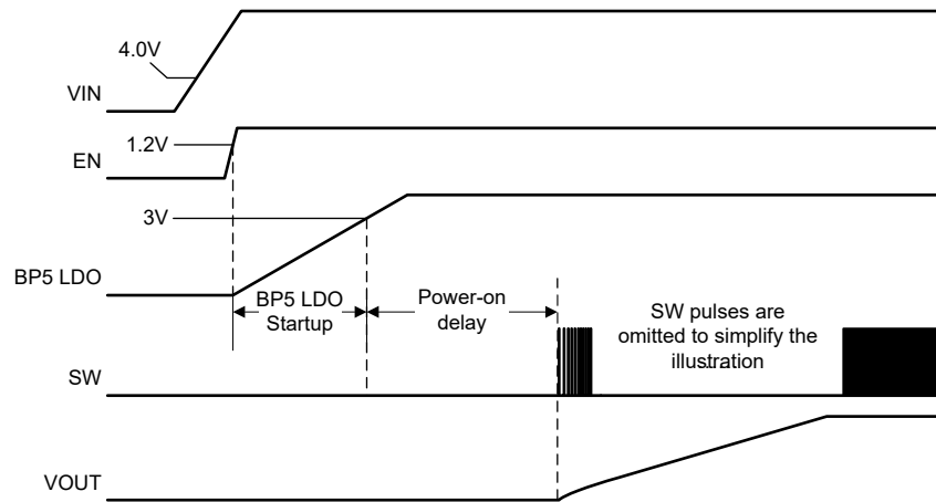
Figure 6-1. Start-Up Sequence
