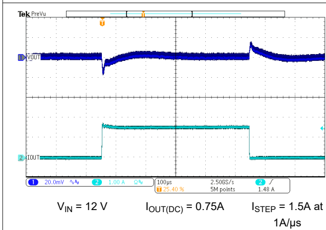
Figure 7-8. Load Transient
