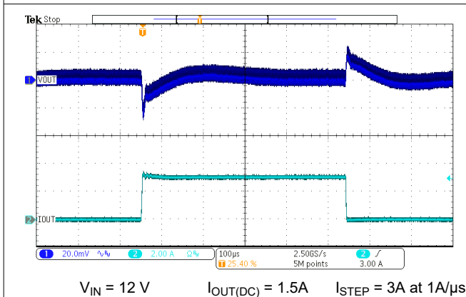
Figure 7-8. Load Transient
