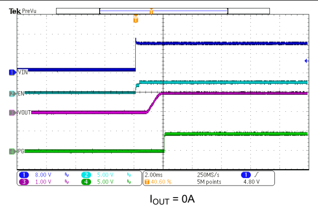
Figure 7-13. VIN Start-Up
