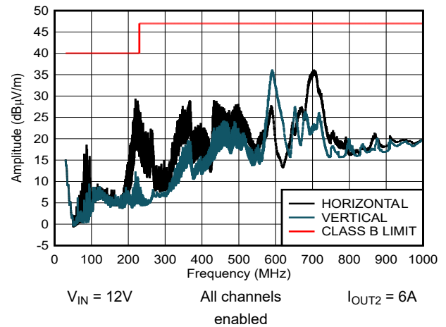
Figure 8-41. Radiated Emissions Test CISPR32 Class B Limits
