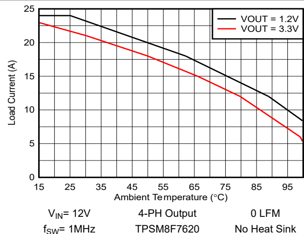
Figure 6-4. Maximum Output Current vs Ambient Temperature
