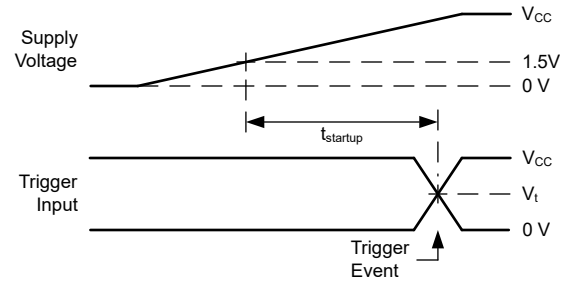
Figure 6-8. Voltage Waveforms, Startup Time
