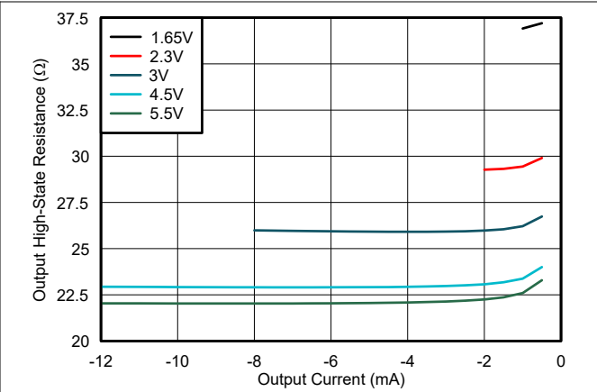
Figure 5-5. Output High-State Resistance vs Output Current
