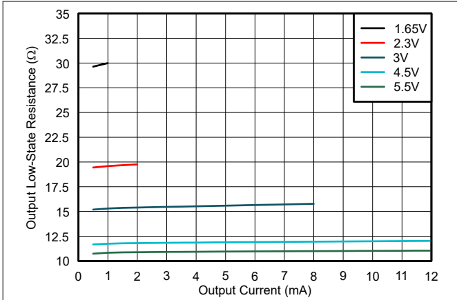
Figure 5-4. Output Low-State Resistance vs Output Current
