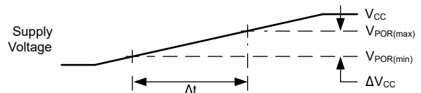
Figure 6-6. Voltage Waveforms, Supply Ramp
