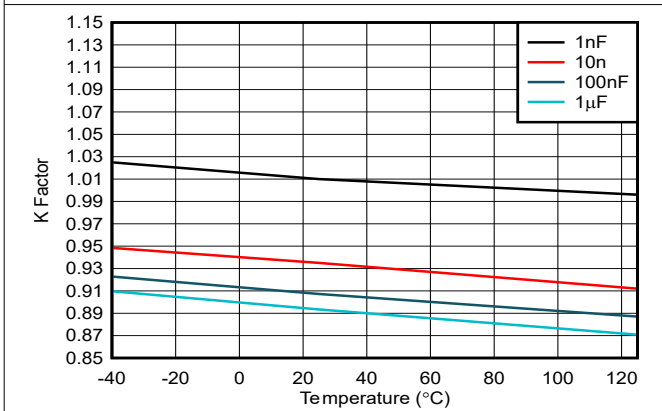
Figure 5-6. K Factor vs Temperature, R_{ext} = 10k\Omega
