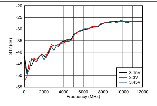
Figure 5-6. Reverse Isolation Across V_{DD}
