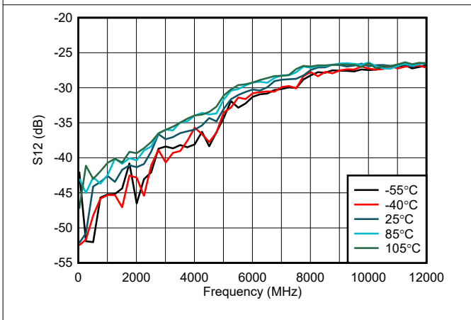
Figure 5-5. Reverse Isolation Across Temperature
