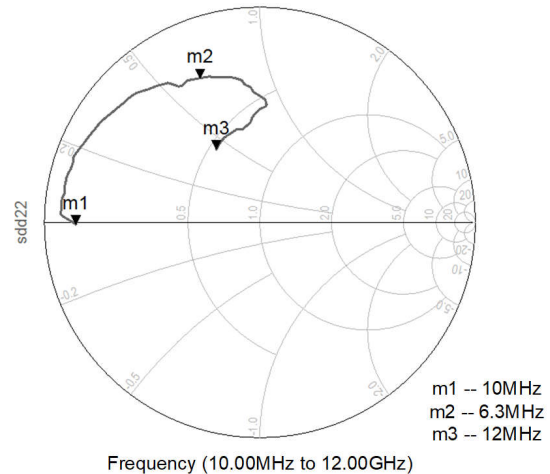
Figure 5-40. Differential S22
