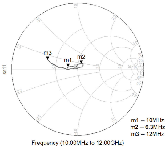
Figure 5-39. Single-Ended S11
