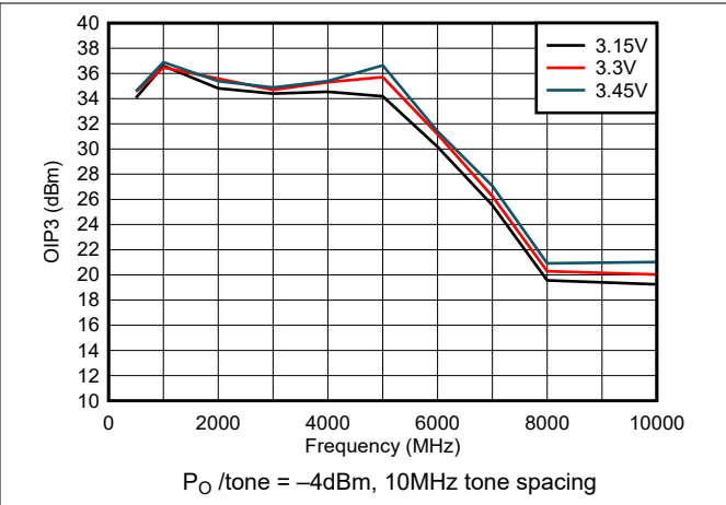
Figure 5-8. OIP3 Across V_{DD}
