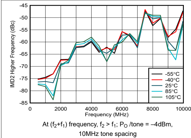
Figure 5-19. IMD2 Higher Across Temperature
