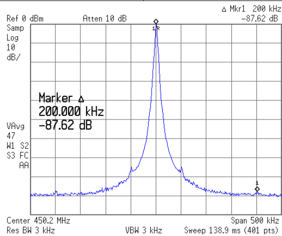
Figure 37. Divide-By-4 Output: PFD Frequency Spurs
