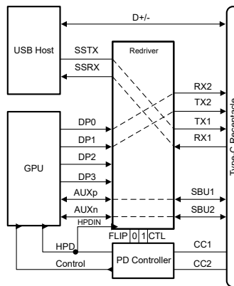
Simplified Schematic
