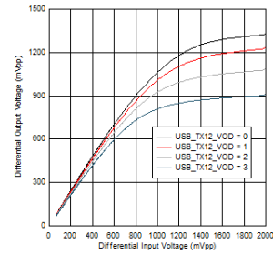
Figure 5-16. USB TX1 VOD Linearity Settings at 100MHz
