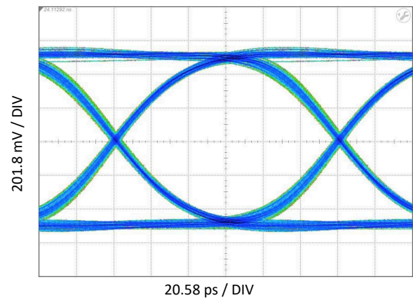
Figure 5-12. DisplayPort HBR3 Eye-Pattern Performance with 12in Input PCB Trace at 8.1Gbps
