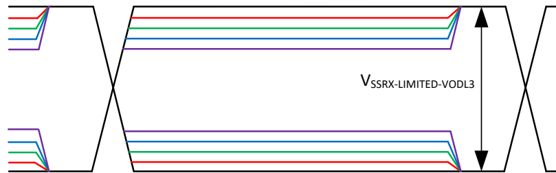
Figure 6-8. SSRX Limited De-emphasis Only
