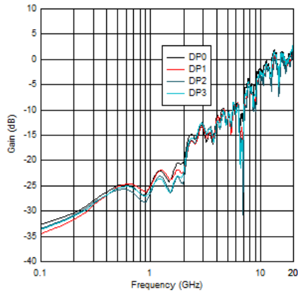
Figure 5-9. DisplayPort Input Return Loss Performance
