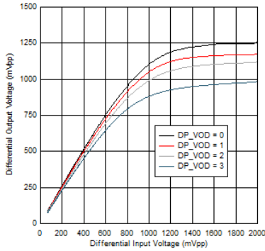
Figure 5-13. DP VOD Linearity Settings at 100MHz
