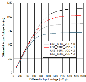
Figure 5-15. USB SSRX VOD Linearity Settings at 100MHz
