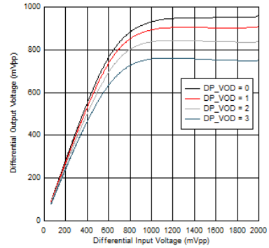
Figure 5-14. DP VOD Linearity Settings at 5GHz
