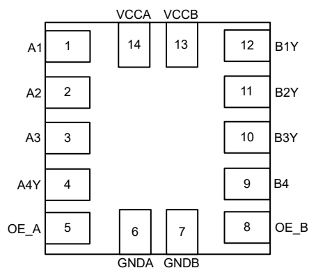
Figure 4-1. TXG1041-Q1 RUC Package 14-Pin X2QFN Top View
