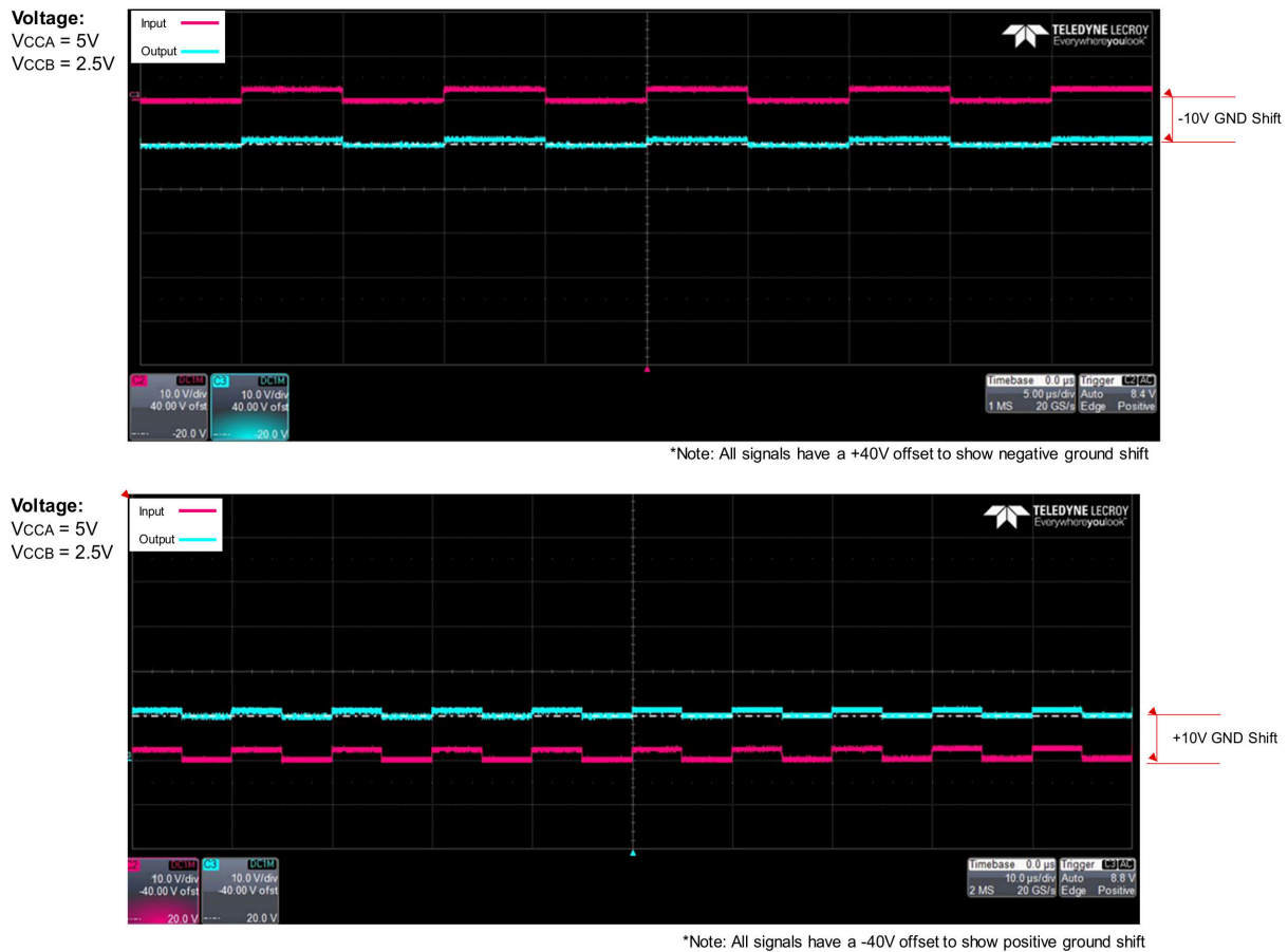
Figure 8-2. Waveform showing -10V (top) and +10V (bottom) Ground Shift with 5V to 2.5V I/O Translation
