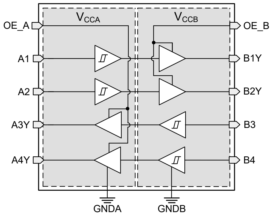
Figure 7-2. TXG1042-Q1 Functional Block Diagram
