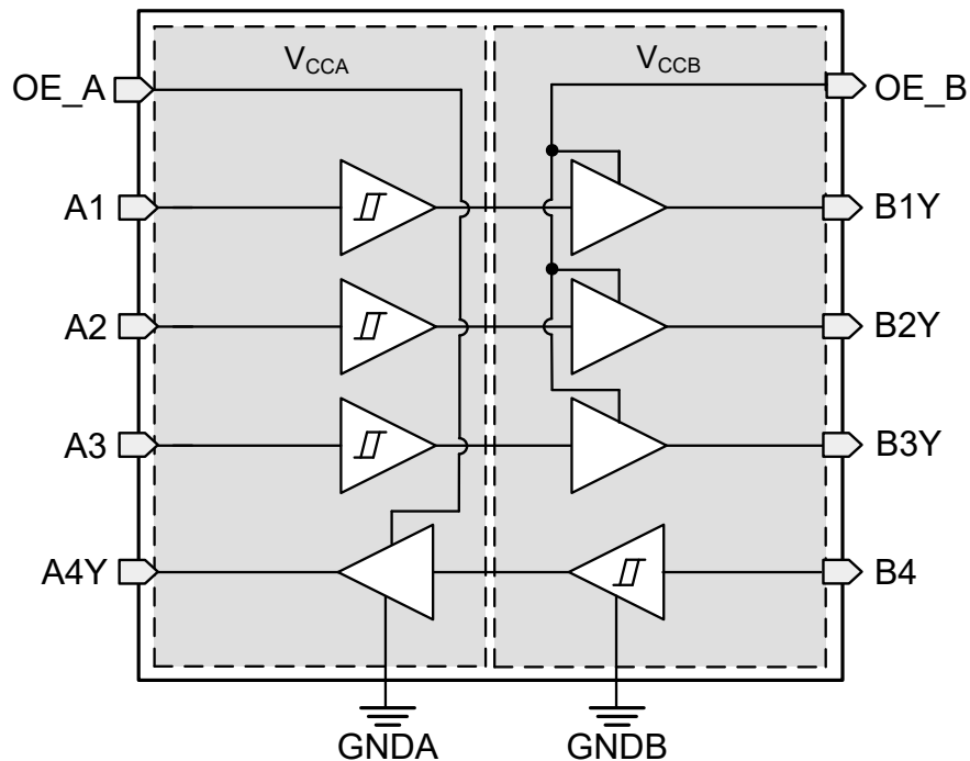
Figure 7-1. TXG1041-Q1 Functional Block Diagram
