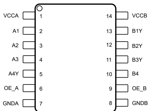
Figure 4-3. TXG1041-Q1 DYY 14-Pin SOT Top View
