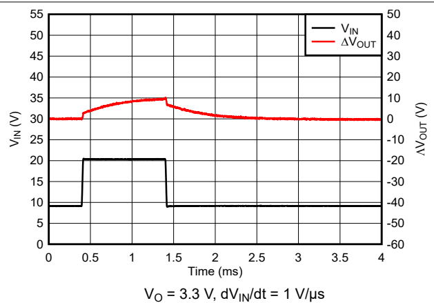
Figure 8-9. Line Transient Behavior for New Chip
