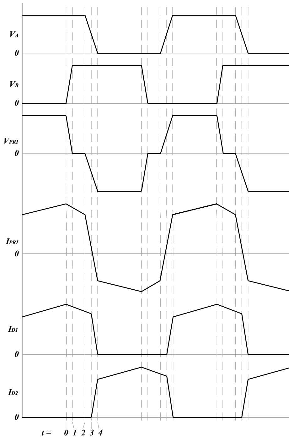
Figure 21. Operational Waveforms
