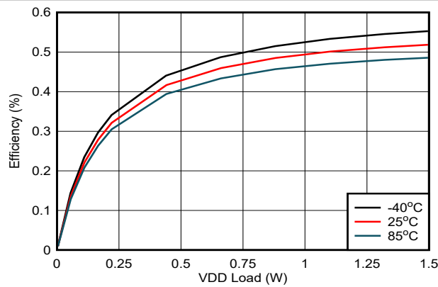
Figure 6-18. Efficiency vs. Load on V_{DD-VEE} : V_{IN} = 13.5V , V_{DD-VEE} = 22V , V_{COM-VEE} = 4V , No Load on V_{COM-VEE}
