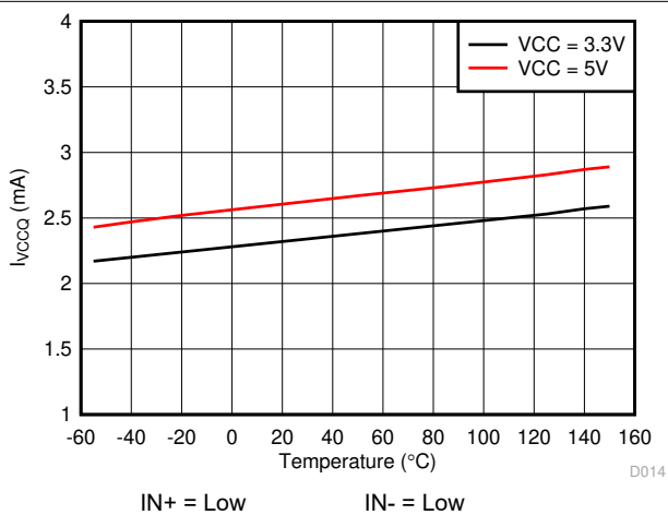
Figure 5-7. I VCCQ Supply Current vs Temperature
