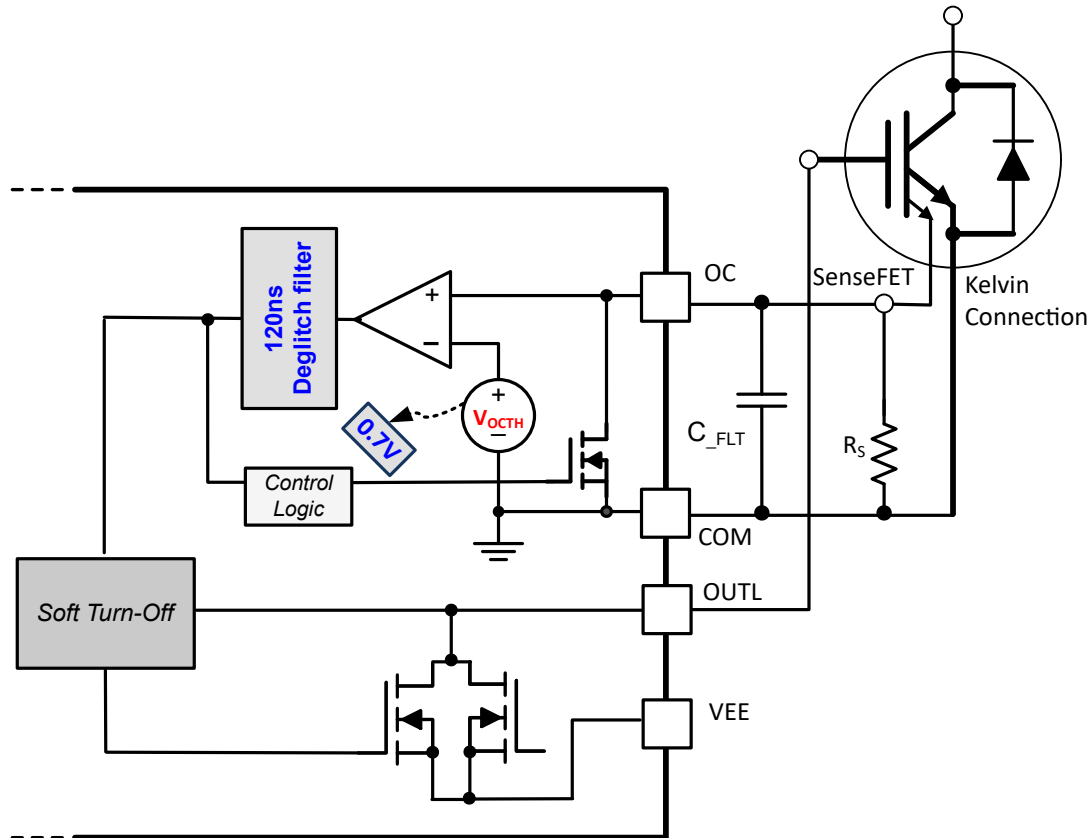
Figure 7-6. Soft Turn-off
