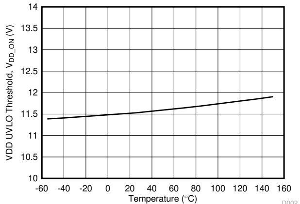
Figure 5-13. VDD UVLO vs Temperature
