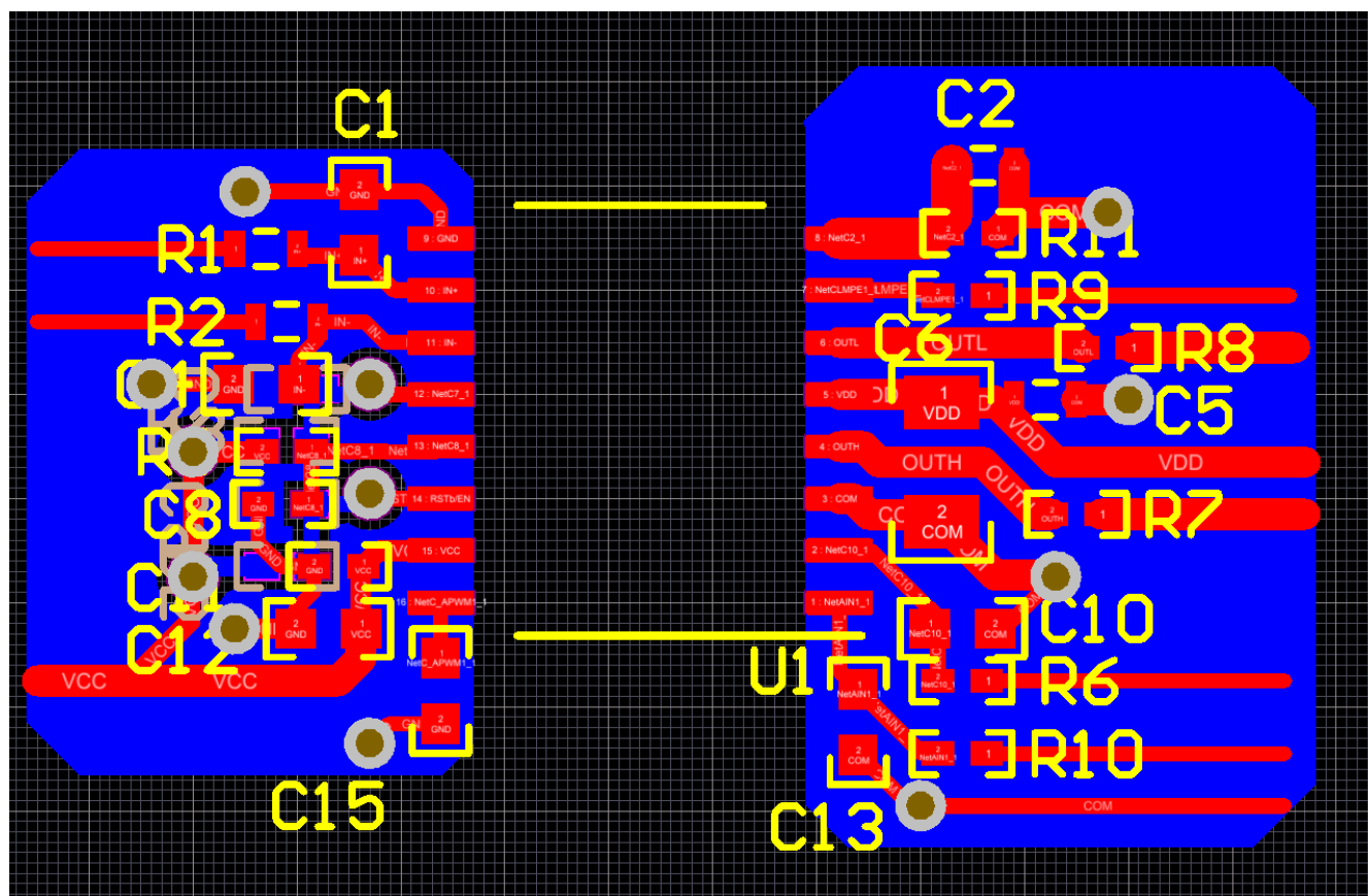
Figure 8-17. Layout Example
