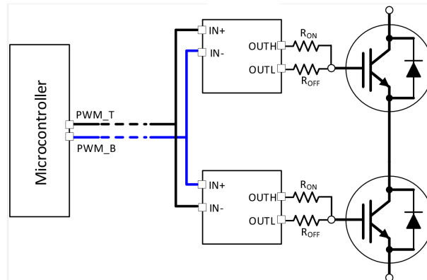
Figure 8-2. PWM Interlock for a Half Bridge
