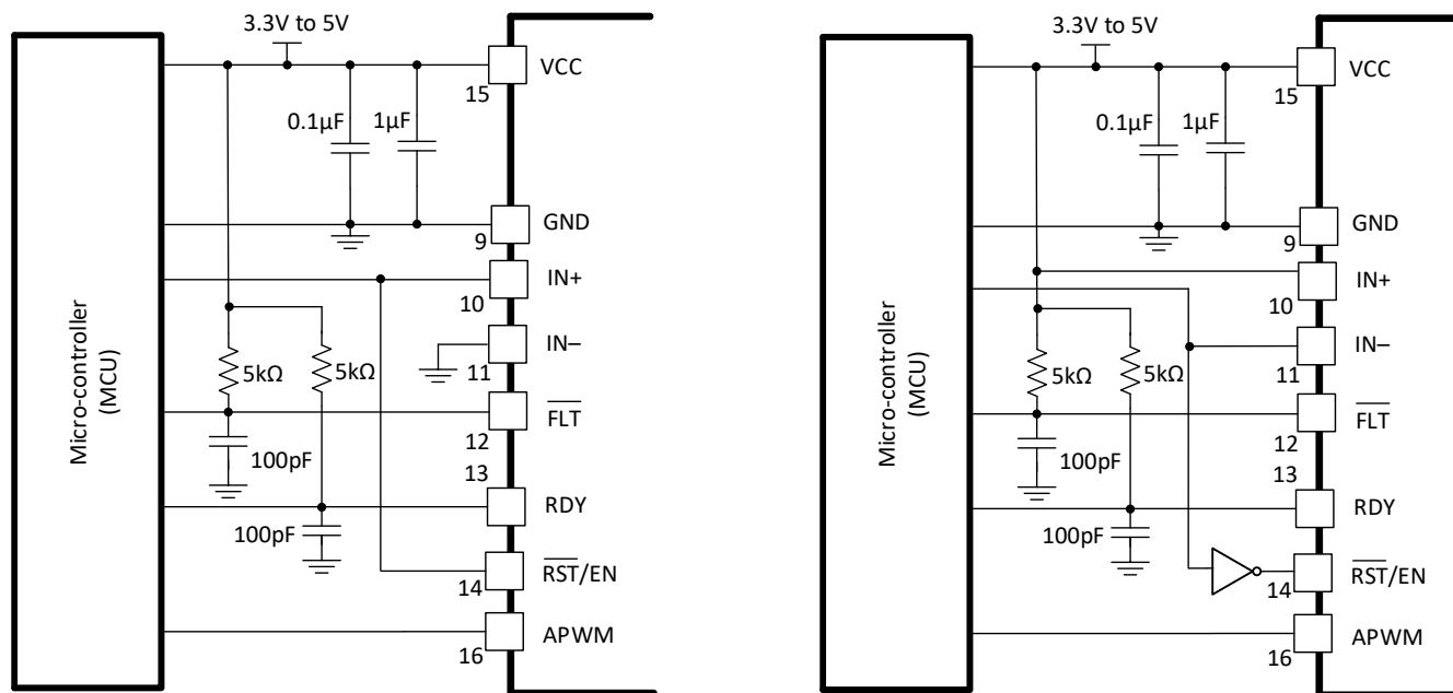
Figure 8-4. Automatic Reset Control
