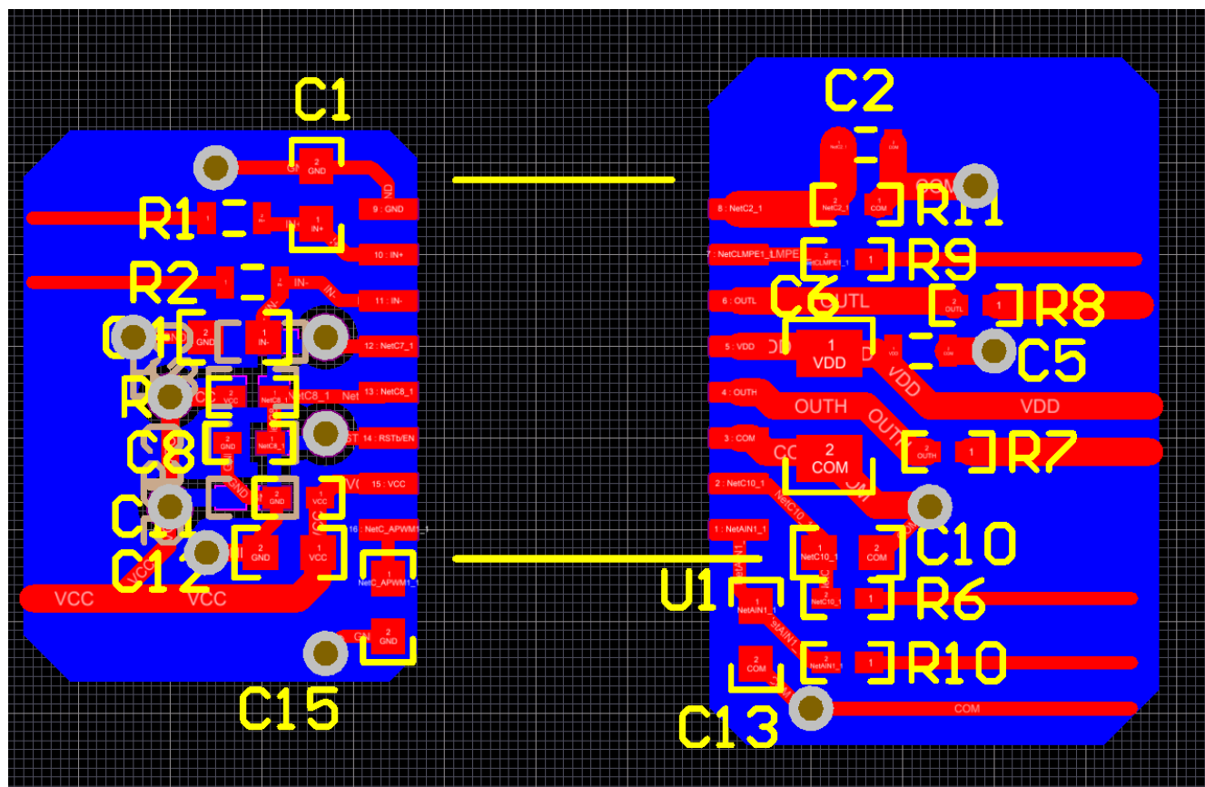
Figure 8-16. Layout Example
